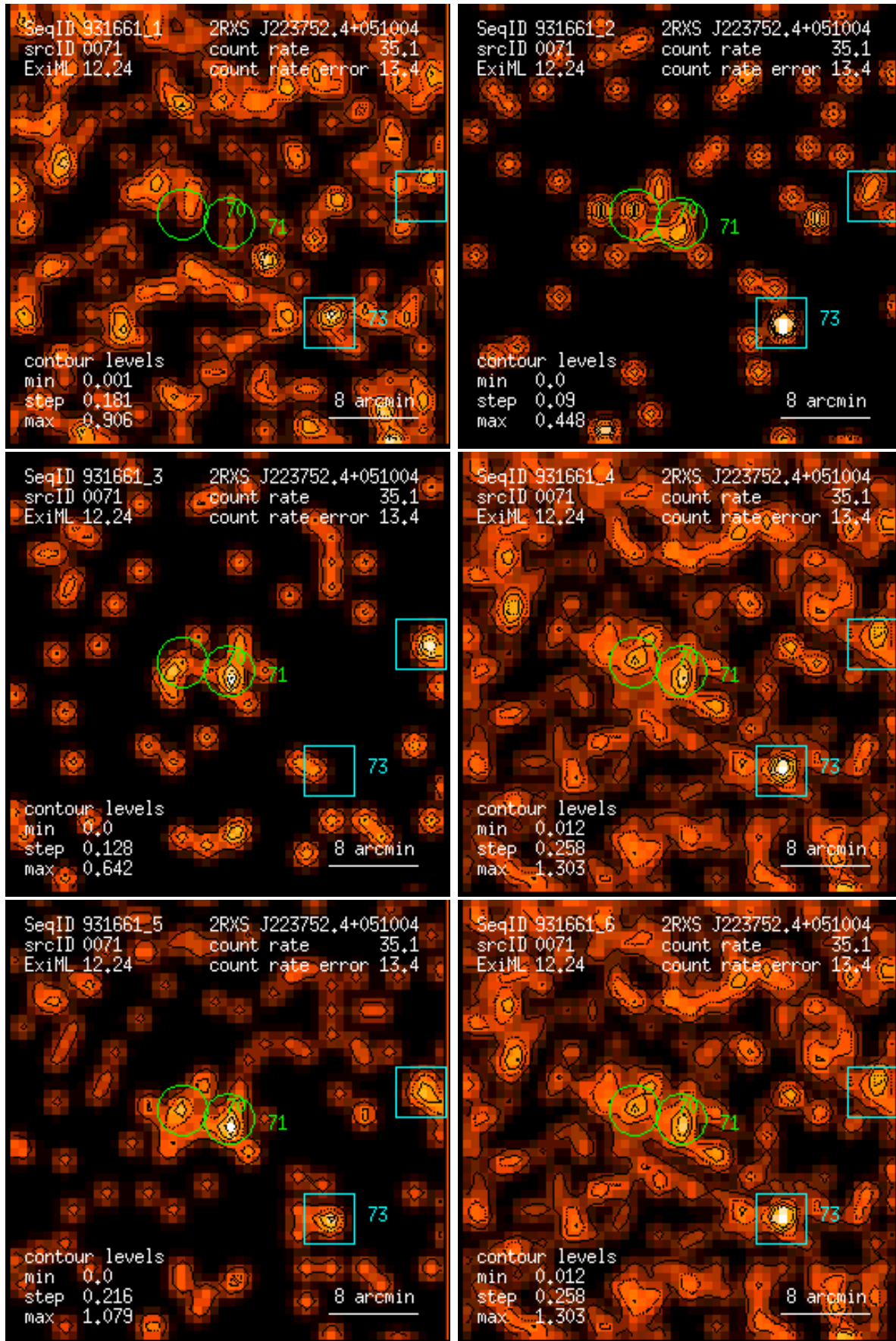
Figure 71: RASS 931661: detection 0071: band rate images, Gaussian filter: (1) PSPC channels 11 – 41, (2) 52 – 90, (3) 91 – 201, (4) 11 – 235, (5) 52 – 201, (6) 11 – 201. Broad band rates in counts/ks. Band rate contour levels in counts/ks/arcmin 2 .
