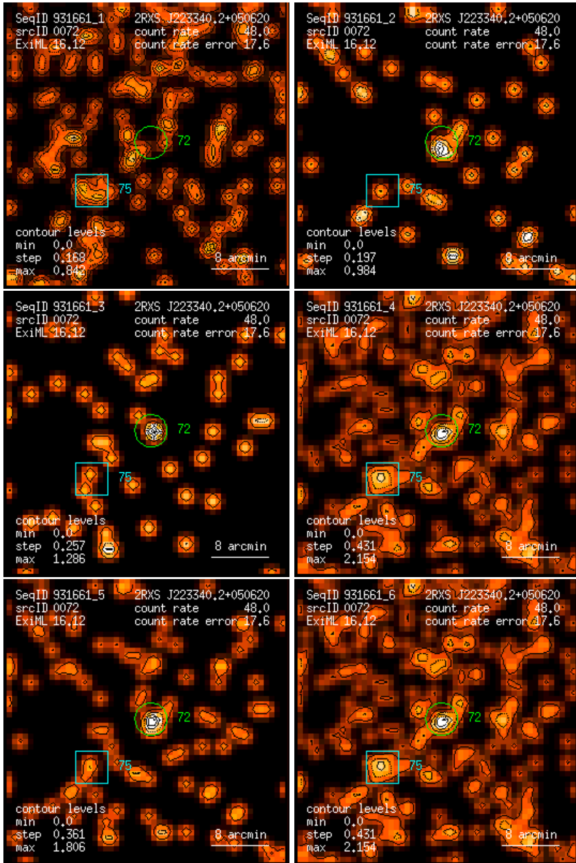
Figure 72: RASS 931661: detection 0072: band rate images, Gaussian filter: (1) PSPC channels 11 – 41, (2) 52 – 90, (3) 91 – 201, (4) 11 – 235, (5) 52 – 201, (6) 11 – 201. Broad band rates in counts/ks. Band rate contour levels in counts/ks/arcmin 2 .
