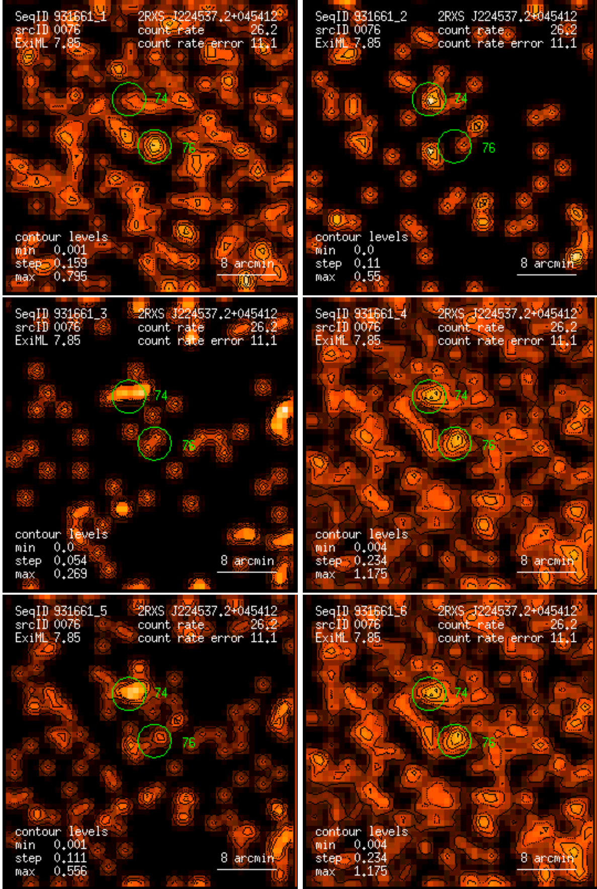
Figure 76: RASS 931661: detection 0076: band rate images, Gaussian filter: (1) PSPC channels 11 – 41, (2) 52 – 90, (3) 91 – 201, (4) 11 – 235, (5) 52 – 201, (6) 11 – 201. Broad band rates in counts/ks. Band rate contour levels in counts/ks/arcmin 2 .
