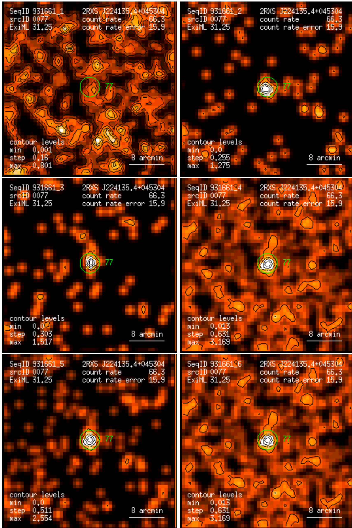
Figure 77: RASS 931661: detection 0077: band rate images, Gaussian filter: (1) PSPC channels 11 – 41, (2) 52 – 90, (3) 91 – 201, (4) 11 – 235, (5) 52 – 201, (6) 11 – 201. Broad band rates in counts/ks. Band rate contour levels in counts/ks/arcmin 2 .
