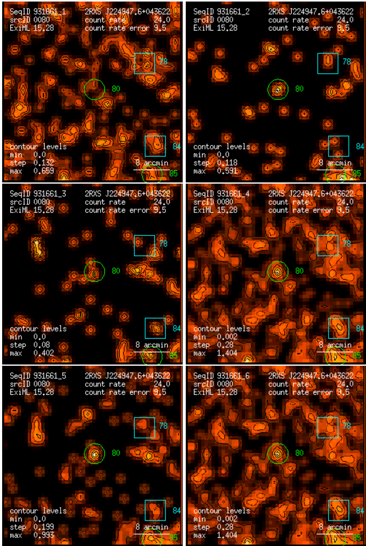
Figure 80: RASS 931661: detection 0080: band rate images, Gaussian filter: (1) PSPC channels 11 – 41, (2) 52 – 90, (3) 91 – 201, (4) 11 – 235, (5) 52 – 201, (6) 11 – 201. Broad band rates in counts/ks. Band rate contour levels in counts/ks/arcmin 2 .
