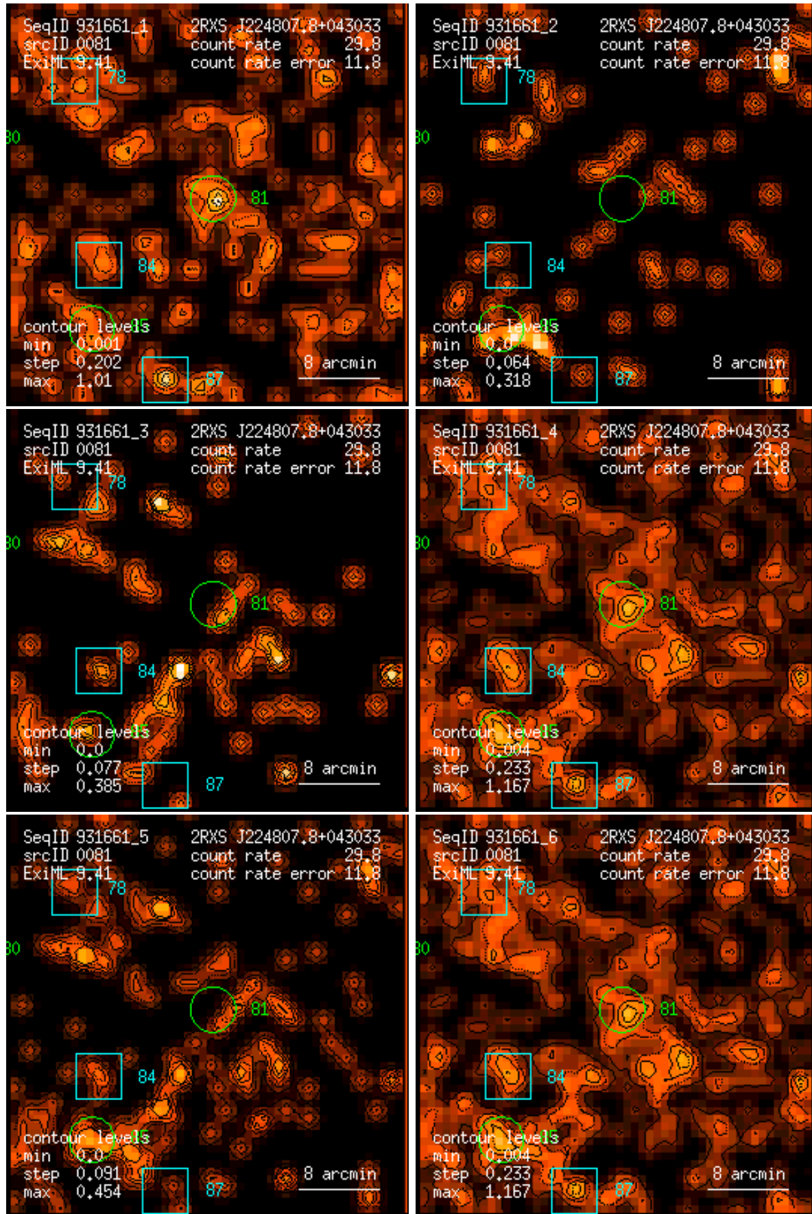
Figure 81: RASS 931661: detection 0081: band rate images, Gaussian filter: (1) PSPC channels 11 – 41, (2) 52 – 90, (3) 91 – 201, (4) 11 – 235, (5) 52 – 201, (6) 11 – 201. Broad band rates in counts/ks. Band rate contour levels in counts/ks/arcmin 2 .
