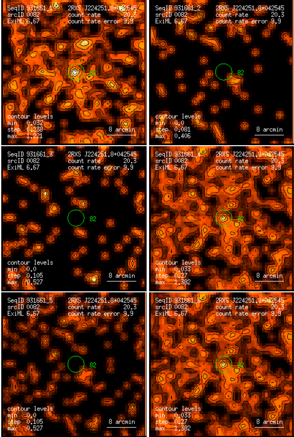
Figure 82: RASS 931661: detection 0082: band rate images, Gaussian filter: (1) PSPC channels 11 – 41, (2) 52 – 90, (3) 91 – 201, (4) 11 – 235, (5) 52 – 201, (6) 11 – 201. Broad band rates in counts/ks. Band rate contour levels in counts/ks/arcmin 2 .
