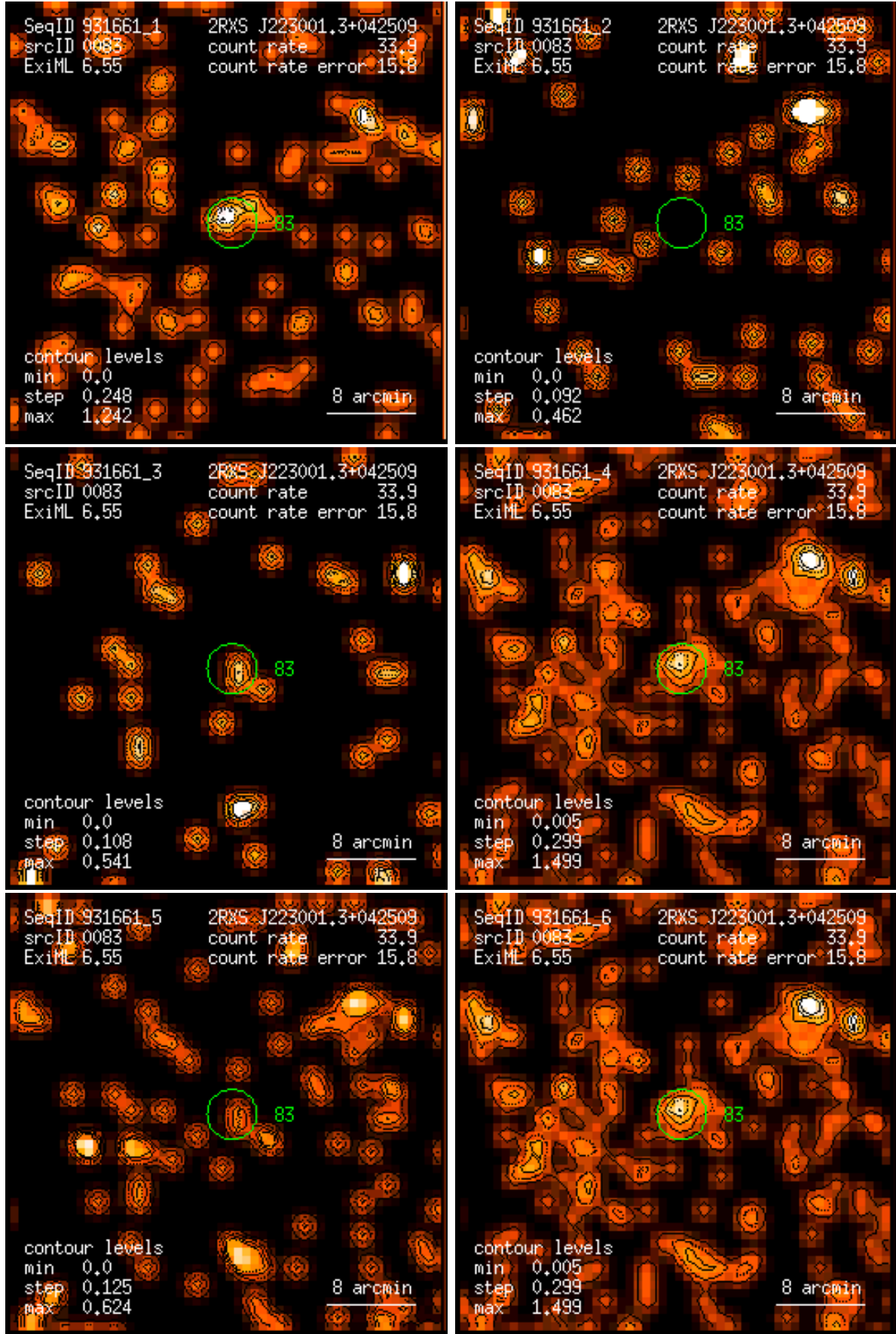
Figure 83: RASS 931661: detection 0083: band rate images, Gaussian filter: (1) PSPC channels 11 – 41, (2) 52 – 90, (3) 91 – 201, (4) 11 – 235, (5) 52 – 201, (6) 11 – 201. Broad band rates in counts/ks. Band rate contour levels in counts/ks/arcmin 2 .
