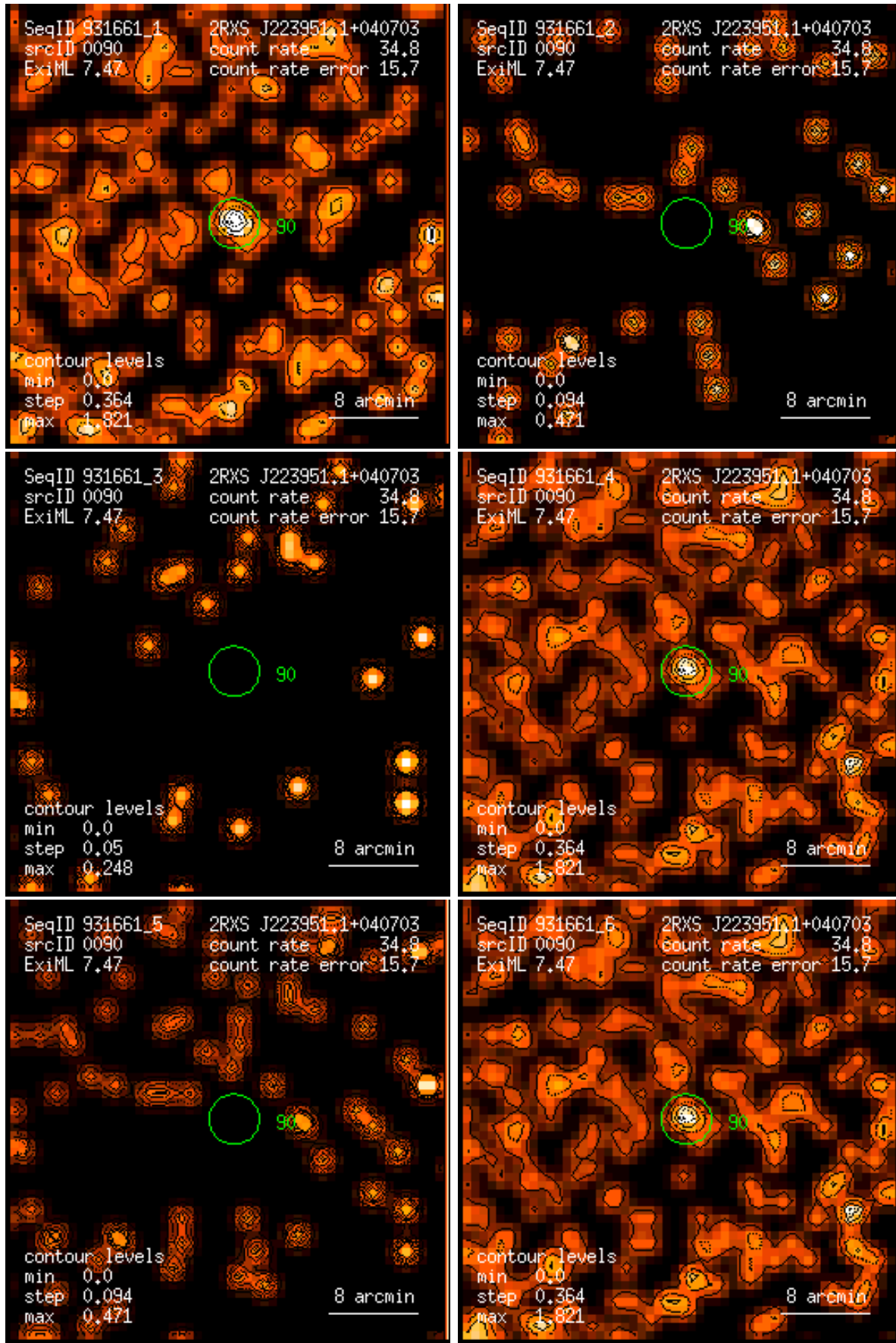
Figure 90: RASS 931661: detection 0090: band rate images, Gaussian filter: (1) PSPC channels 11 – 41, (2) 52 – 90, (3) 91 – 201, (4) 11 – 235, (5) 52 – 201, (6) 11 – 201. Broad band rates in counts/ks. Band rate contour levels in counts/ks/arcmin 2 .
