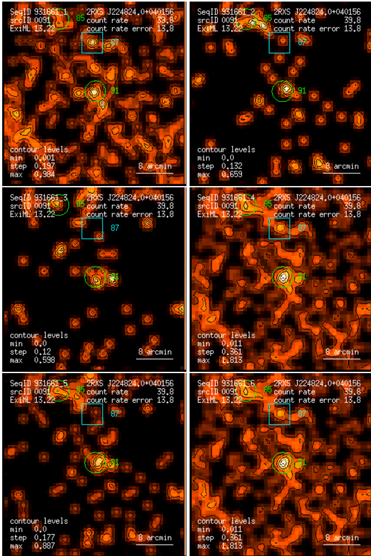
Figure 91: RASS 931661: detection 0091: band rate images, Gaussian filter: (1) PSPC channels 11 – 41, (2) 52 – 90, (3) 91 – 201, (4) 11 – 235, (5) 52 – 201, (6) 11 – 201. Broad band rates in counts/ks. Band rate contour levels in counts/ks/arcmin 2 .
