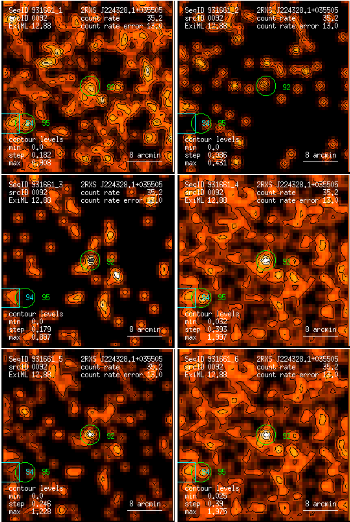
Figure 92: RASS 931661: detection 0092: band rate images, Gaussian filter: (1) PSPC channels 11 – 41, (2) 52 – 90, (3) 91 – 201, (4) 11 – 235, (5) 52 – 201, (6) 11 – 201. Broad band rates in counts/ks. Band rate contour levels in counts/ks/arcmin 2 .
