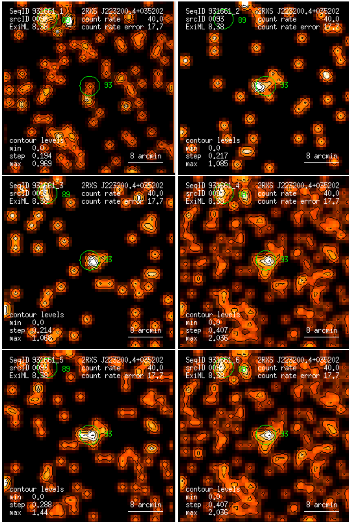
Figure 93: RASS 931661: detection 0093: band rate images, Gaussian filter: (1) PSPC channels 11 – 41, (2) 52 – 90, (3) 91 – 201, (4) 11 – 235, (5) 52 – 201, (6) 11 – 201. Broad band rates in counts/ks. Band rate contour levels in counts/ks/arcmin 2 .
