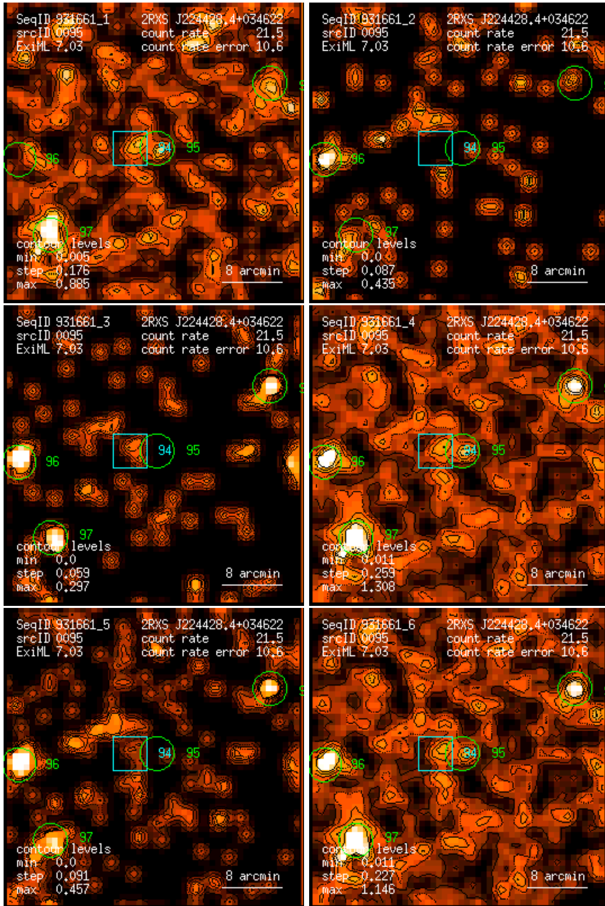
Figure 95: RASS 931661: detection 0095: band rate images, Gaussian filter: (1) PSPC channels 11 – 41, (2) 52 – 90, (3) 91 – 201, (4) 11 – 235, (5) 52 – 201, (6) 11 – 201. Broad band rates in counts/ks. Band rate contour levels in counts/ks/arcmin 2 .
