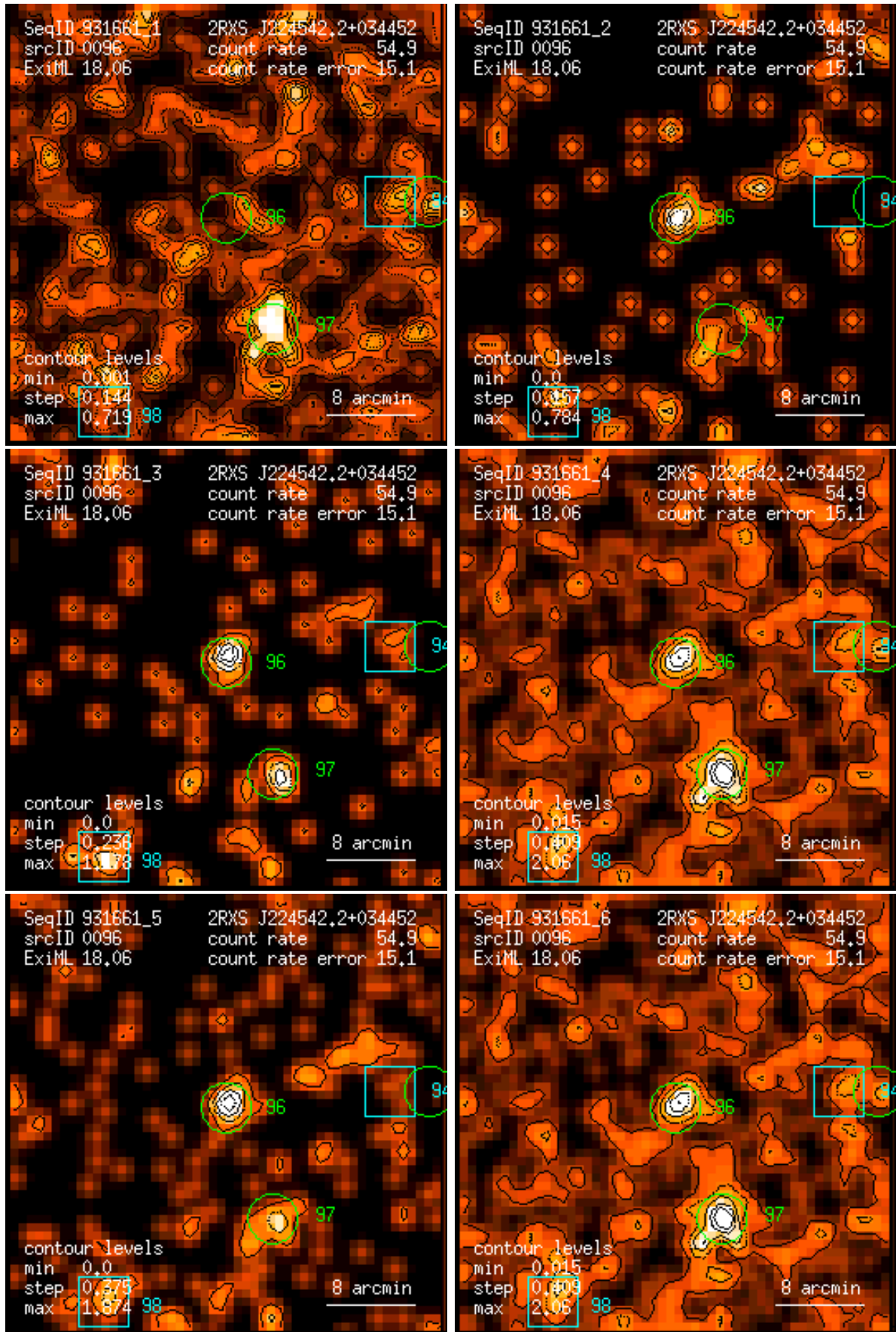
Figure 96: RASS 931661: detection 0096: band rate images, Gaussian filter: (1) PSPC channels 11 – 41, (2) 52 – 90, (3) 91 – 201, (4) 11 – 235, (5) 52 – 201, (6) 11 – 201. Broad band rates in counts/ks. Band rate contour levels in counts/ks/arcmin 2 .
