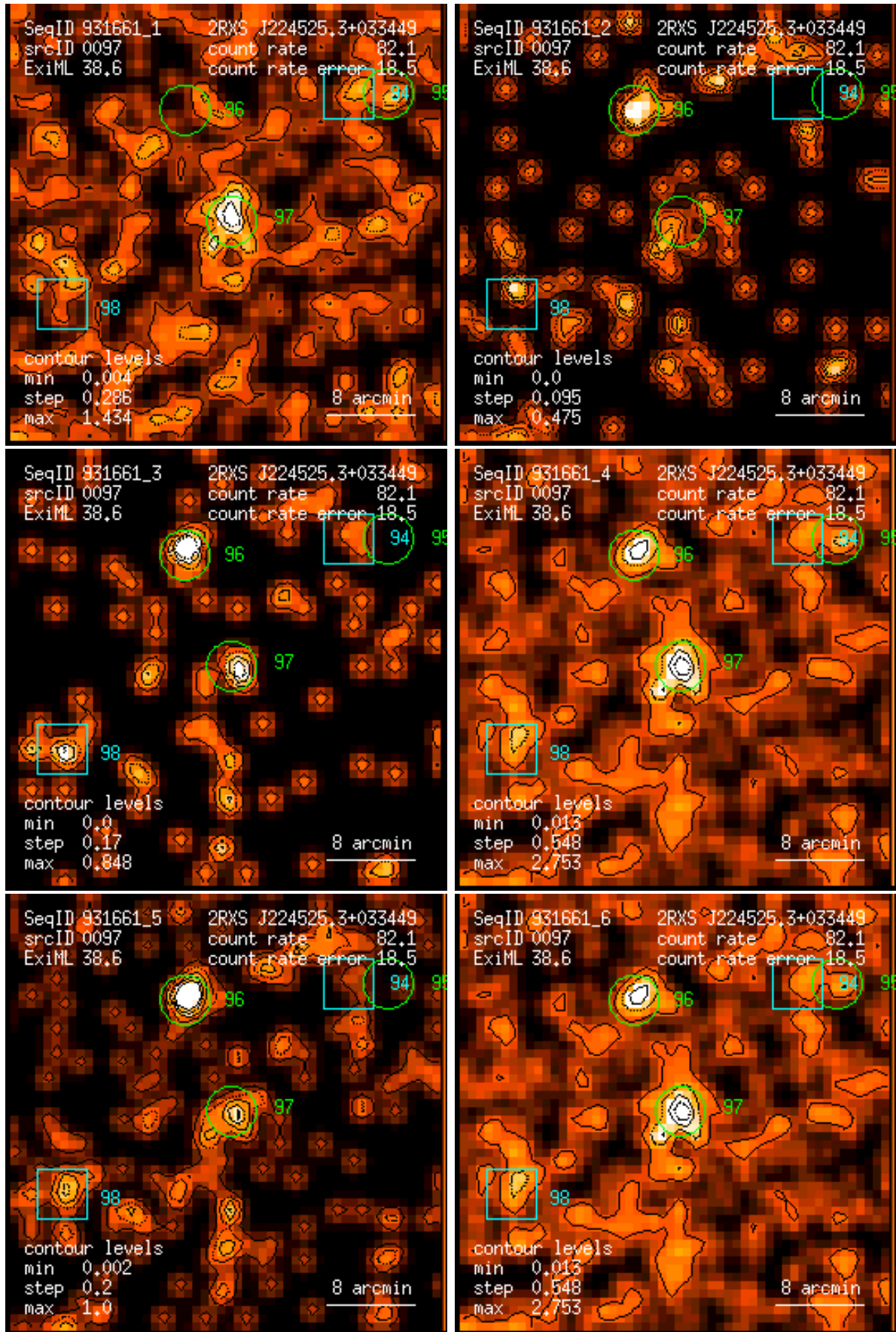
Figure 97: RASS 931661: detection 0097: band rate images, Gaussian filter: (1) PSPC channels 11 – 41, (2) 52 – 90, (3) 91 – 201, (4) 11 – 235, (5) 52 – 201, (6) 11 – 201. Broad band rates in counts/ks. Band rate contour levels in counts/ks/arcmin 2 .
