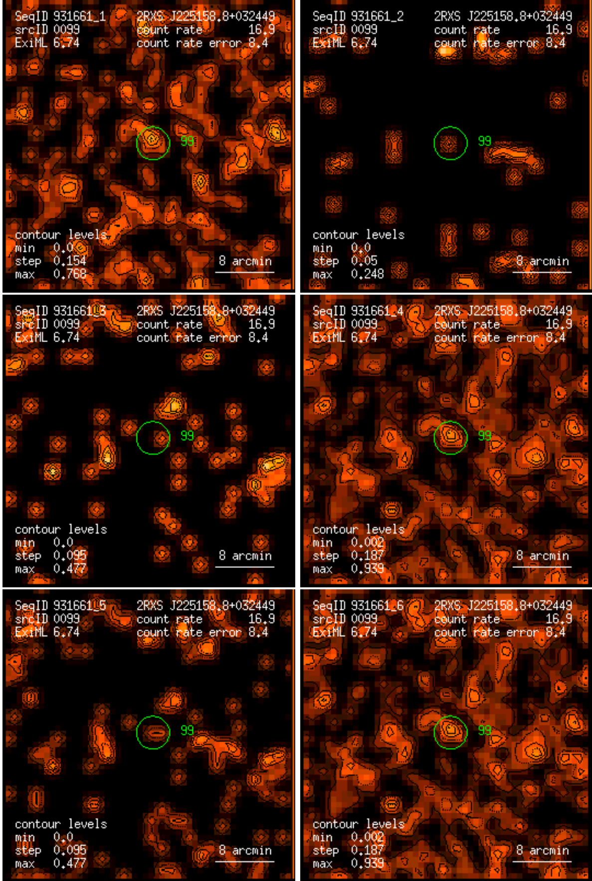
Figure 99: RASS 931661: detection 0099: band rate images, Gaussian filter: (1) PSPC channels 11 – 41, (2) 52 – 90, (3) 91 – 201, (4) 11 – 235, (5) 52 – 201, (6) 11 – 201. Broad band rates in counts/ks. Band rate contour levels in counts/ks/arcmin 2 .
