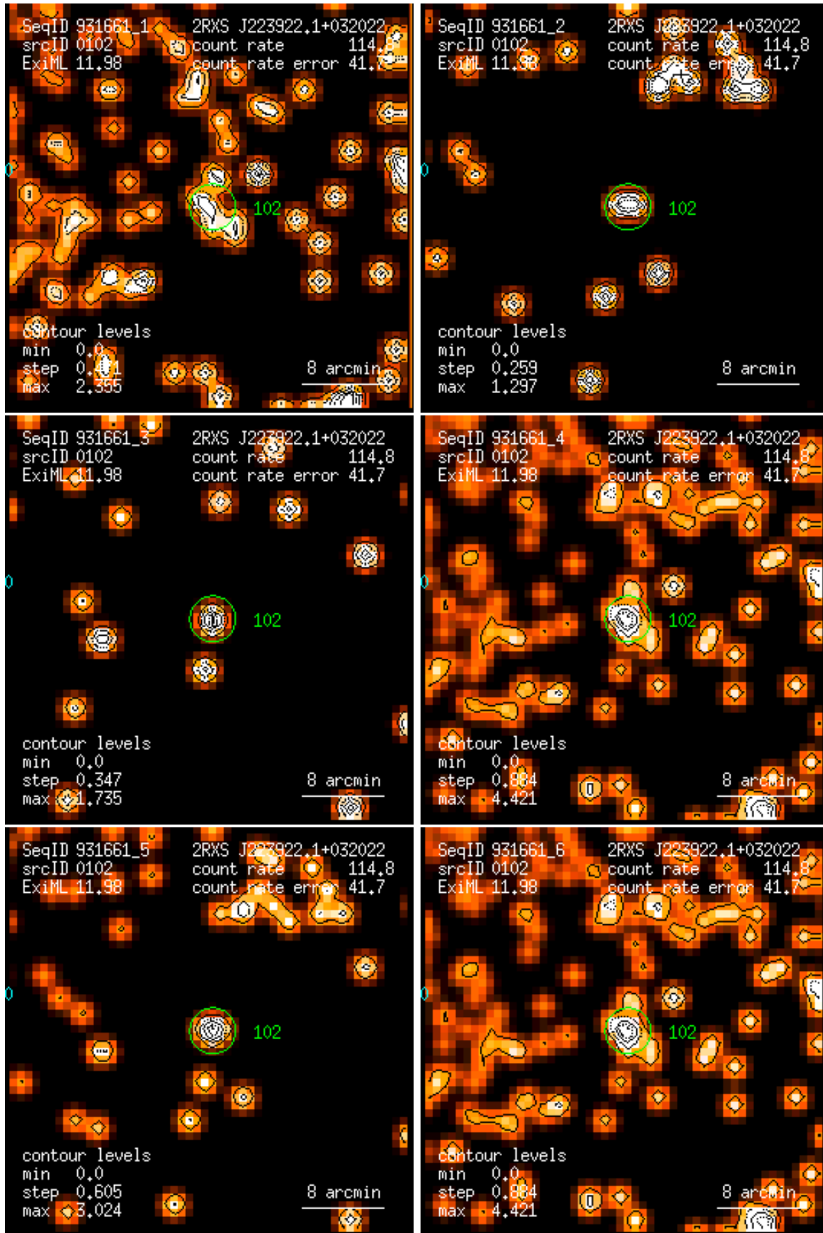
Figure 102: RASS 931661: detection 0102: band rate images, Gaussian filter: (1) PSPC channels 11 – 41, (2) 52 – 90, (3) 91 – 201, (4) 11 – 235, (5) 52 – 201, (6) 11 – 201. Broad band rates in counts/ks. Band rate contour levels in counts/ks/arcmin 2 .
