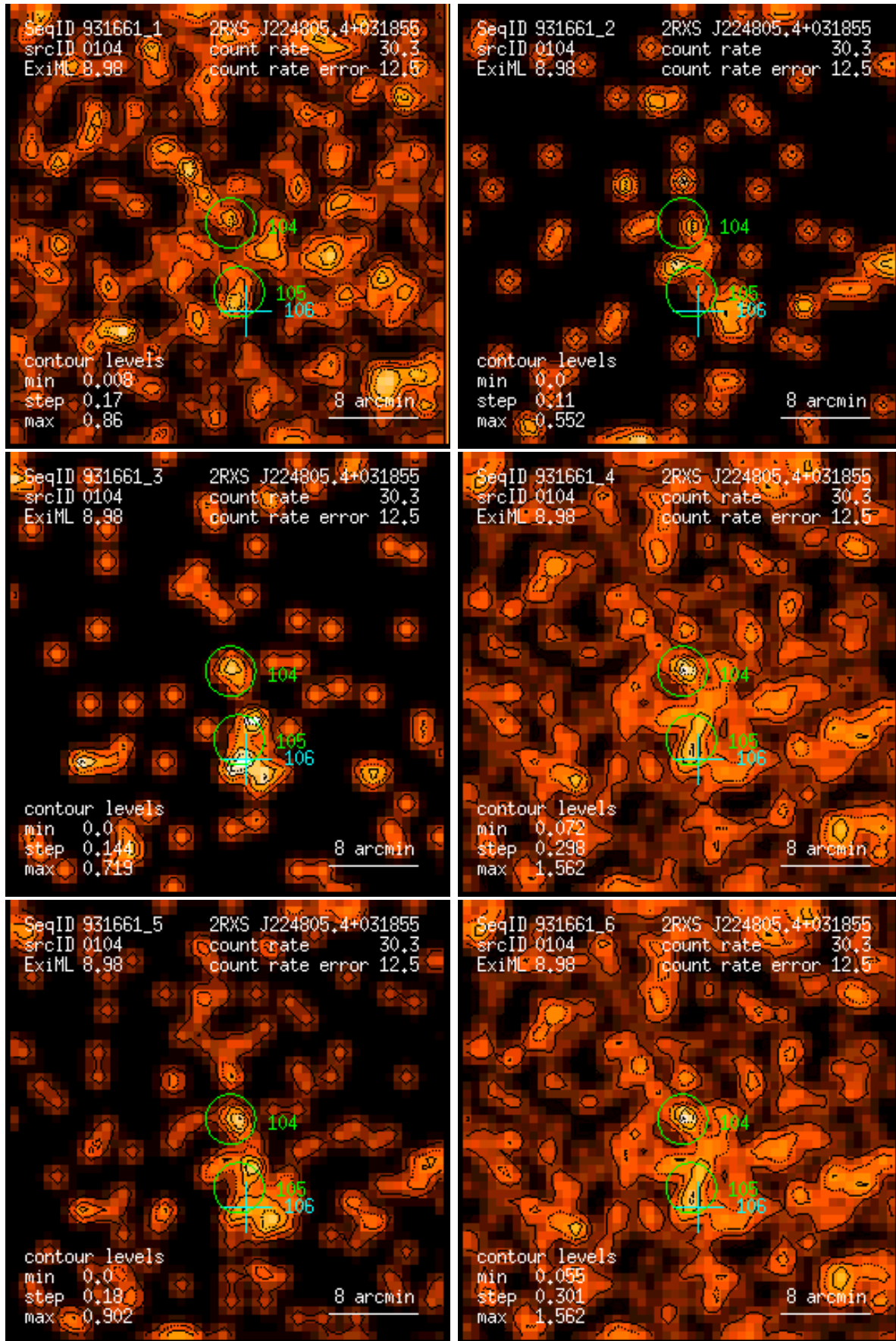
Figure 104: RASS 931661: detection 0104: band rate images, Gaussian filter: (1) PSPC channels 11 – 41, (2) 52 – 90, (3) 91 – 201, (4) 11 – 235, (5) 52 – 201, (6) 11 – 201. Broad band rates in counts/ks. Band rate contour levels in counts/ks/arcmin 2 .
