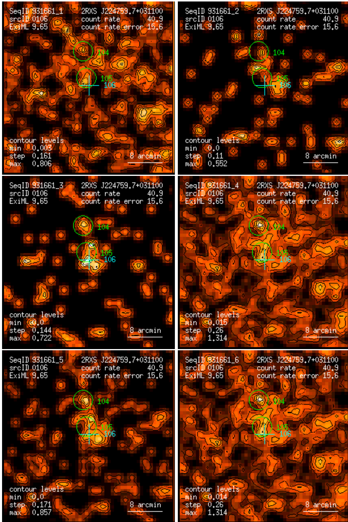
Figure 106: RASS 931661: detection 0106: band rate images, Gaussian filter: (1) PSPC channels 11 – 41, (2) 52 – 90, (3) 91 – 201, (4) 11 – 235, (5) 52 – 201, (6) 11 – 201. Broad band rates in counts/ks. Band rate contour levels in counts/ks/arcmin 2 .
