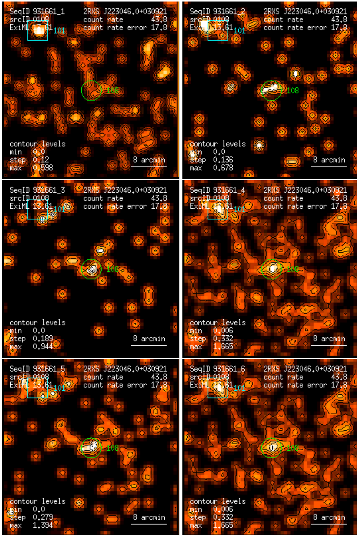
Figure 108: RASS 931661: detection 0108: band rate images, Gaussian filter: (1) PSPC channels 11 – 41, (2) 52 – 90, (3) 91 – 201, (4) 11 – 235, (5) 52 – 201, (6) 11 – 201. Broad band rates in counts/ks. Band rate contour levels in counts/ks/arcmin 2 .
