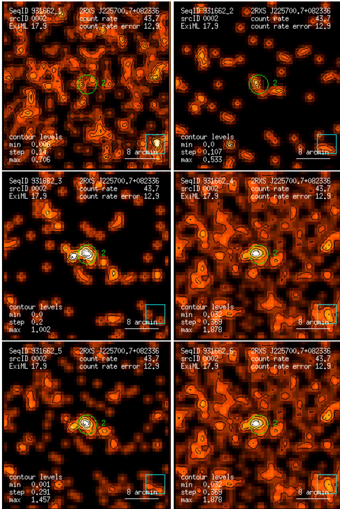
Figure 2: RASS 931662: detection 0002: band rate images, Gaussian filter: (1) PSPC channels 11 – 41, (2) 52 – 90, (3) 91 – 201, (4) 11 – 235, (5) 52 – 201, (6) 11 – 201. Broad band rates in counts/ks. Band rate contour levels in counts/ks/arcmin 2 .
