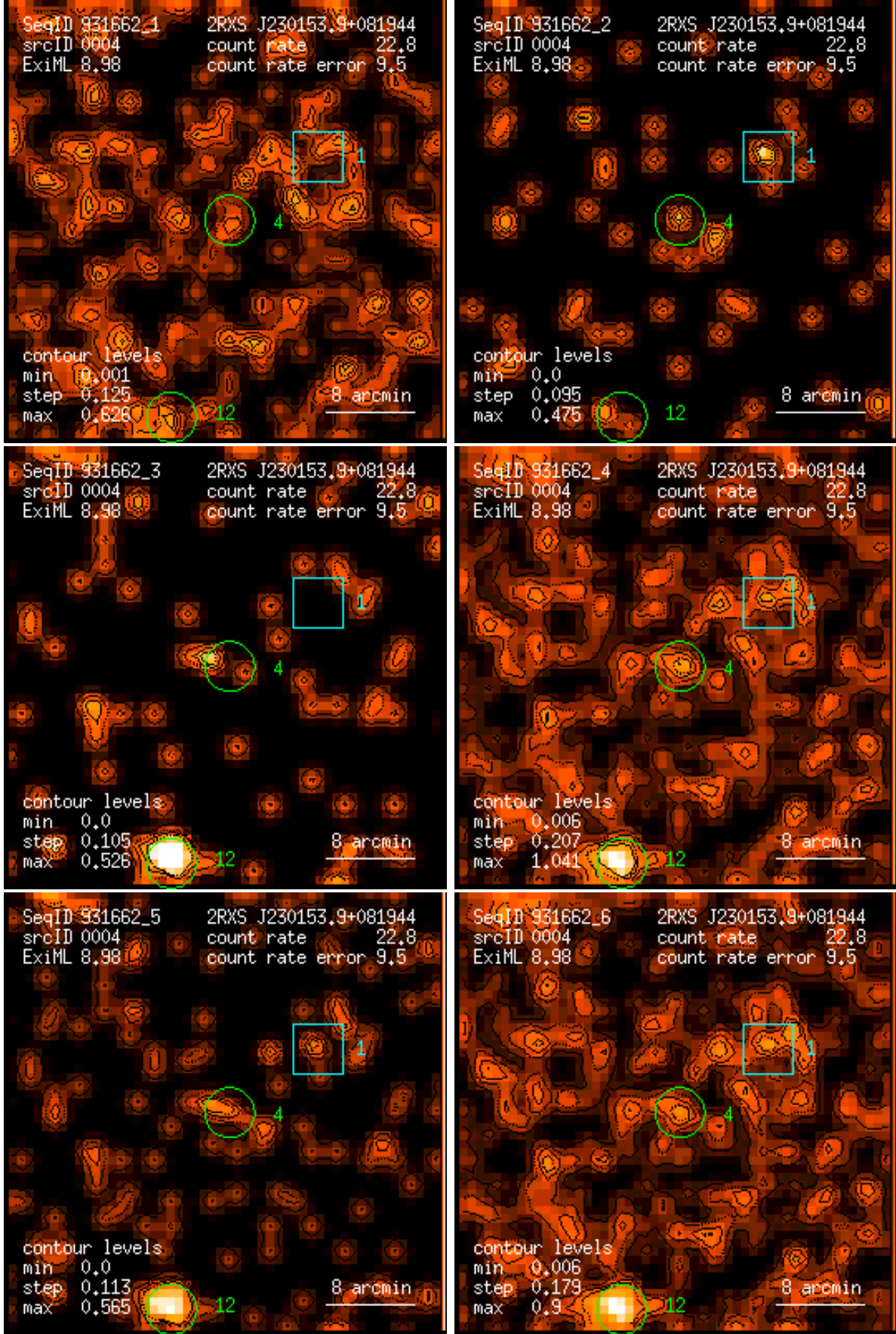
Figure 4: RASS 931662: detection 0004: band rate images, Gaussian filter: (1) PSPC channels 11 – 41, (2) 52 – 90, (3) 91 – 201, (4) 11 – 235, (5) 52 – 201, (6) 11 – 201. Broad band rates in counts/ks. Band rate contour levels in counts/ks/arcmin 2 .
