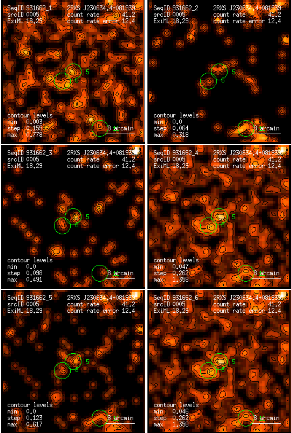
Figure 5: RASS 931662: detection 0005: band rate images, Gaussian filter: (1) PSPC channels 11 – 41, (2) 52 – 90, (3) 91 – 201, (4) 11 – 235, (5) 52 – 201, (6) 11 – 201. Broad band rates in counts/ks. Band rate contour levels in counts/ks/arcmin 2 .
