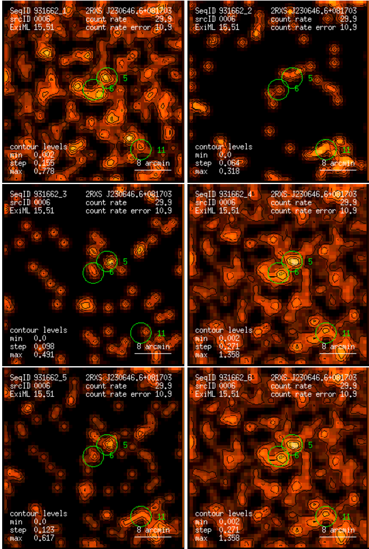
Figure 6: RASS 931662: detection 0006: band rate images, Gaussian filter: (1) PSPC channels 11 – 41, (2) 52 – 90, (3) 91 – 201, (4) 11 – 235, (5) 52 – 201, (6) 11 – 201. Broad band rates in counts/ks. Band rate contour levels in counts/ks/arcmin 2 .
