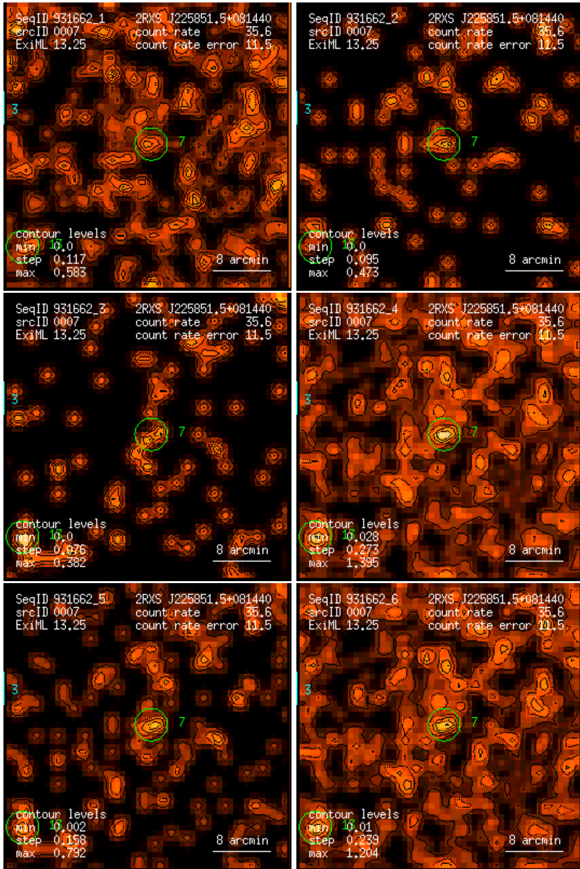
Figure 7: RASS 931662: detection 0007: band rate images, Gaussian filter: (1) PSPC channels 11 – 41, (2) 52 – 90, (3) 91 – 201, (4) 11 – 235, (5) 52 – 201, (6) 11 – 201. Broad band rates in counts/ks. Band rate contour levels in counts/ks/arcmin 2 .
