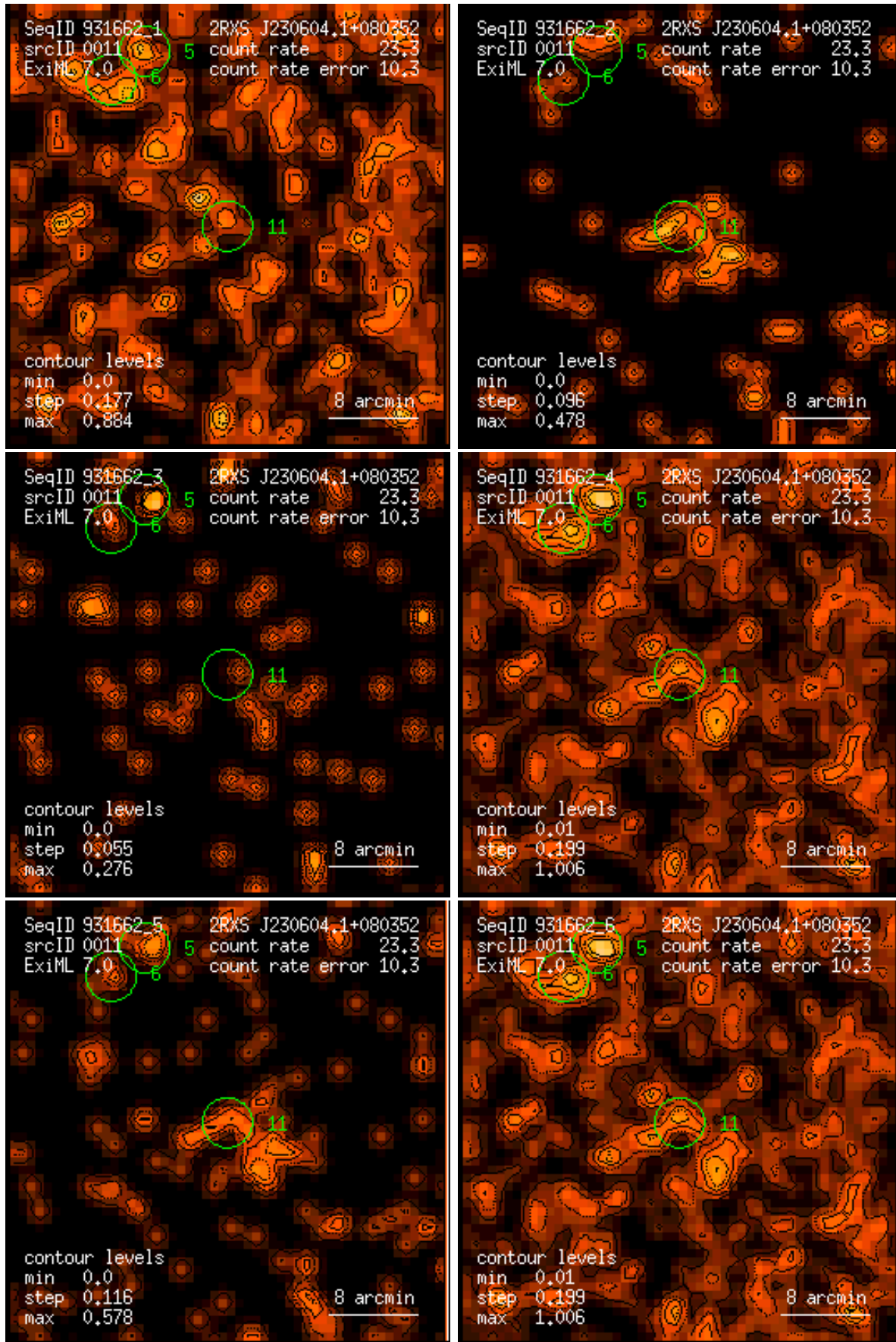
Figure 11: RASS 931662: detection 0011: band rate images, Gaussian filter: (1) PSPC channels 11 – 41, (2) 52 – 90, (3) 91 – 201, (4) 11 – 235, (5) 52 – 201, (6) 11 – 201. Broad band rates in counts/ks. Band rate contour levels in counts/ks/arcmin 2 .
