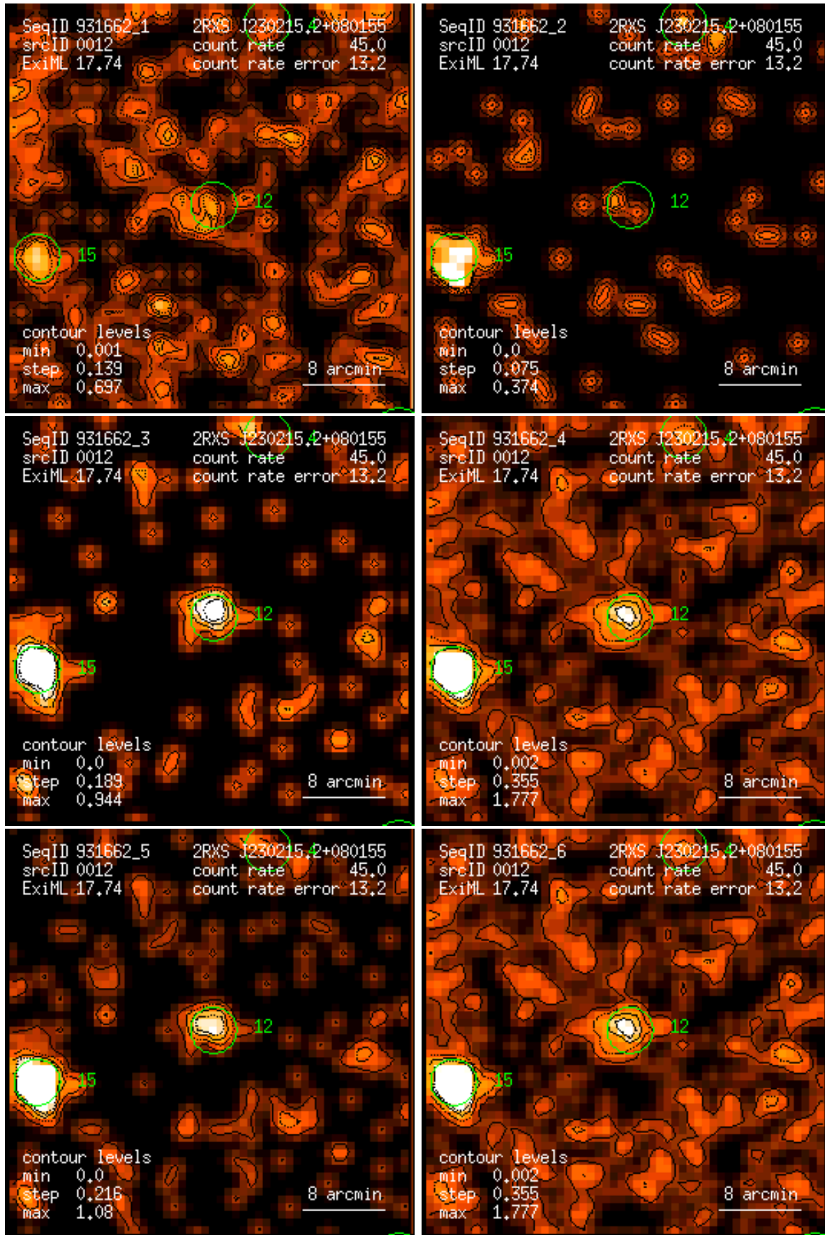
Figure 12: RASS 931662: detection 0012: band rate images, Gaussian filter: (1) PSPC channels 11 – 41, (2) 52 – 90, (3) 91 – 201, (4) 11 – 235, (5) 52 – 201, (6) 11 – 201. Broad band rates in counts/ks. Band rate contour levels in counts/ks/arcmin 2 .
