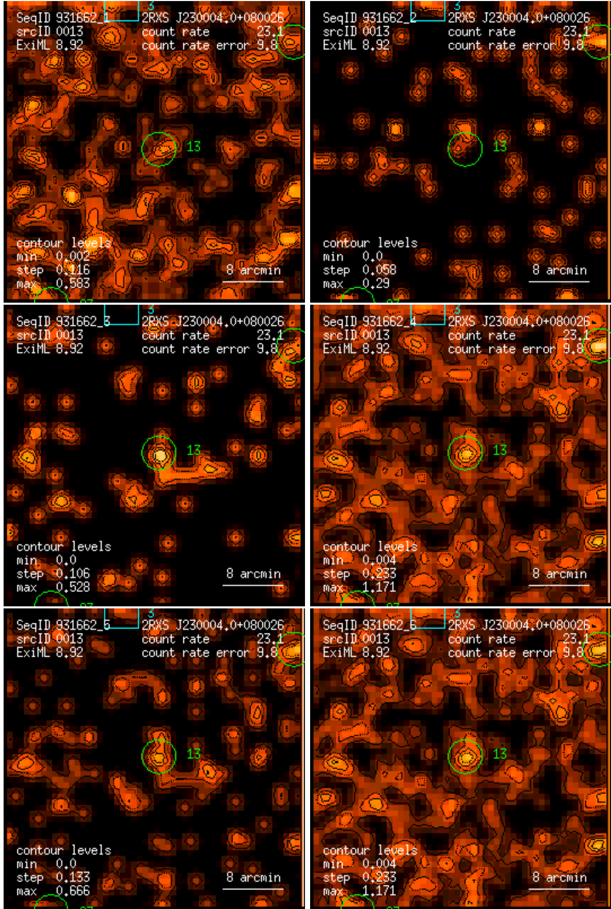
Figure 13: RASS 931662: detection 0013: band rate images, Gaussian filter: (1) PSPC channels 11 – 41, (2) 52 – 90, (3) 91 – 201, (4) 11 – 235, (5) 52 – 201, (6) 11 – 201. Broad band rates in counts/ks. Band rate contour levels in counts/ks/arcmin 2 .
