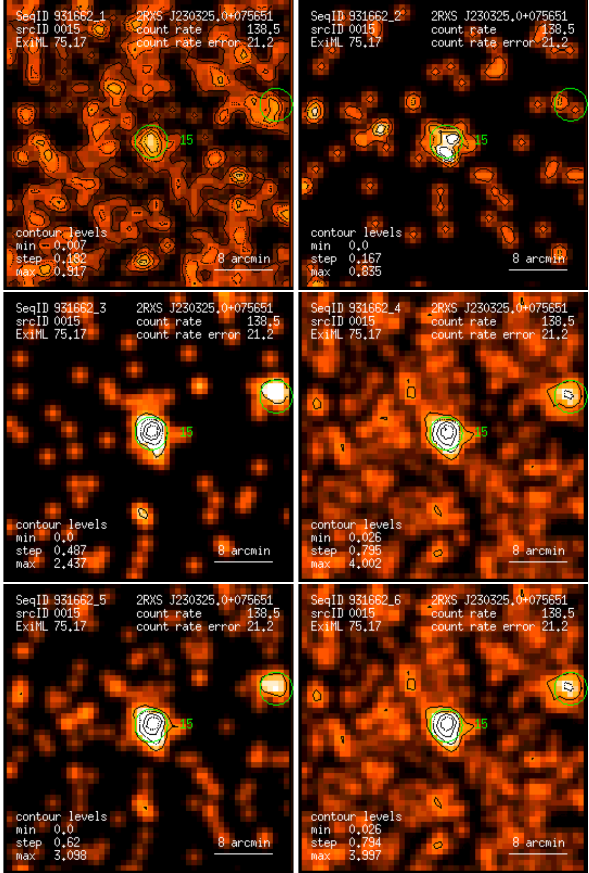
Figure 15: RASS 931662: detection 0015: band rate images, Gaussian filter: (1) PSPC channels 11 – 41, (2) 52 – 90, (3) 91 – 201, (4) 11 – 235, (5) 52 – 201, (6) 11 – 201. Broad band rates in counts/ks. Band rate contour levels in counts/ks/arcmin 2 .
