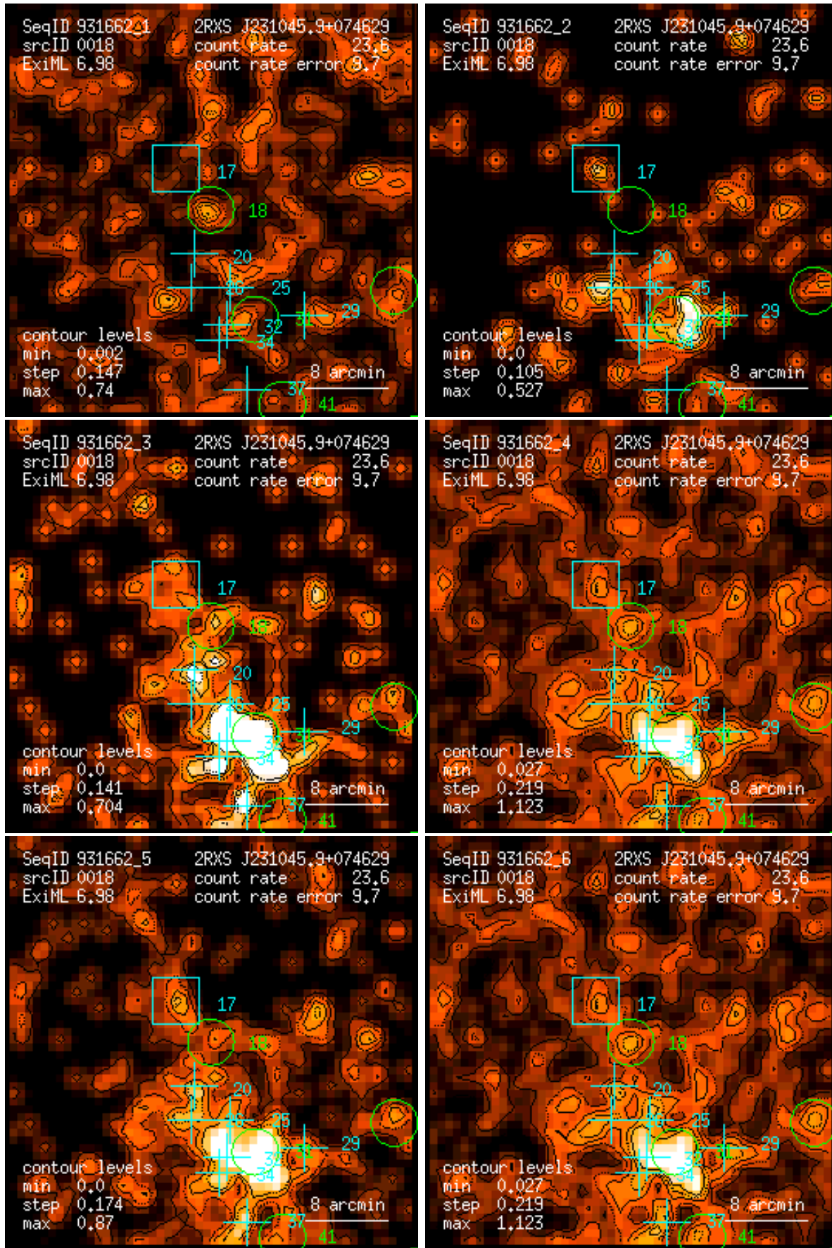
Figure 18: RASS 931662: detection 0018: band rate images, Gaussian filter: (1) PSPC channels 11 – 41, (2) 52 – 90, (3) 91 – 201, (4) 11 – 235, (5) 52 – 201, (6) 11 – 201. Broad band rates in counts/ks. Band rate contour levels in counts/ks/arcmin 2 .
