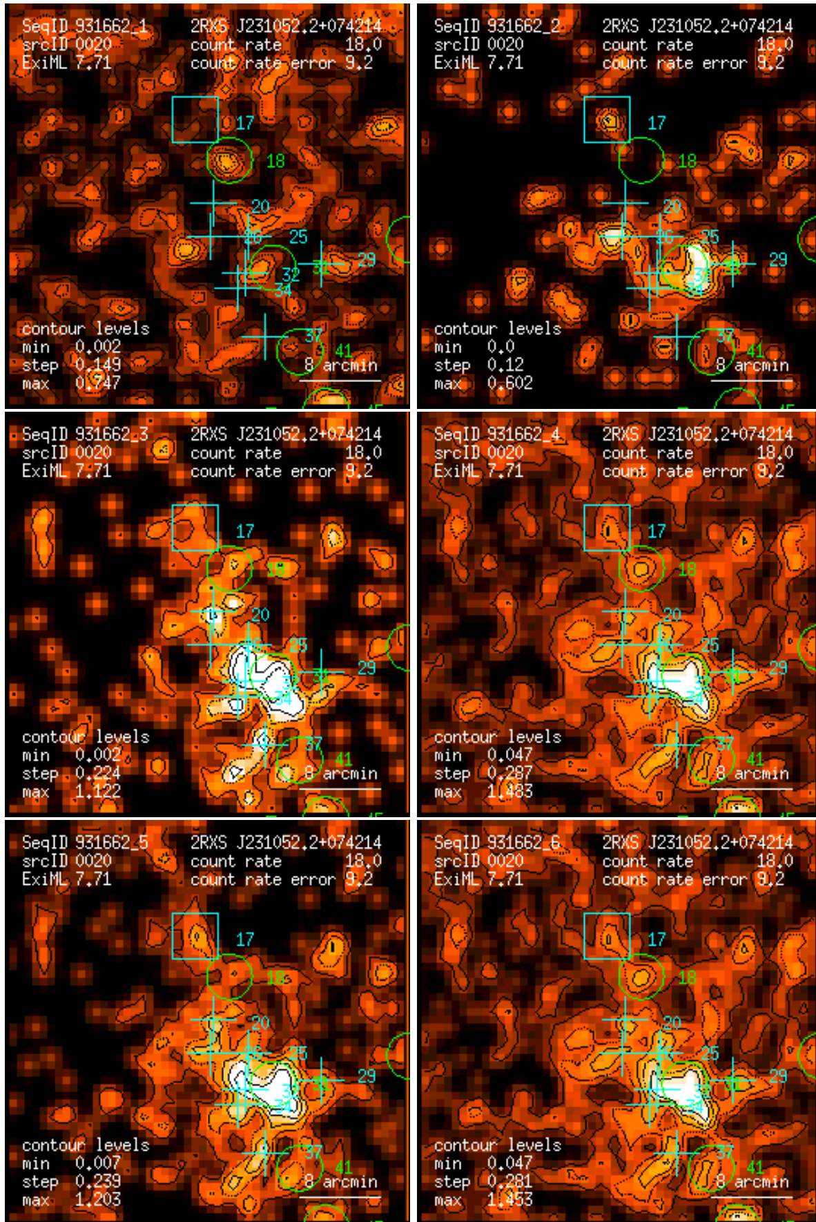
Figure 20: RASS 931662: detection 0020: band rate images, Gaussian filter: (1) PSPC channels 11 – 41, (2) 52 – 90, (3) 91 – 201, (4) 11 – 235, (5) 52 – 201, (6) 11 – 201. Broad band rates in counts/ks. Band rate contour levels in counts/ks/arcmin 2 .
