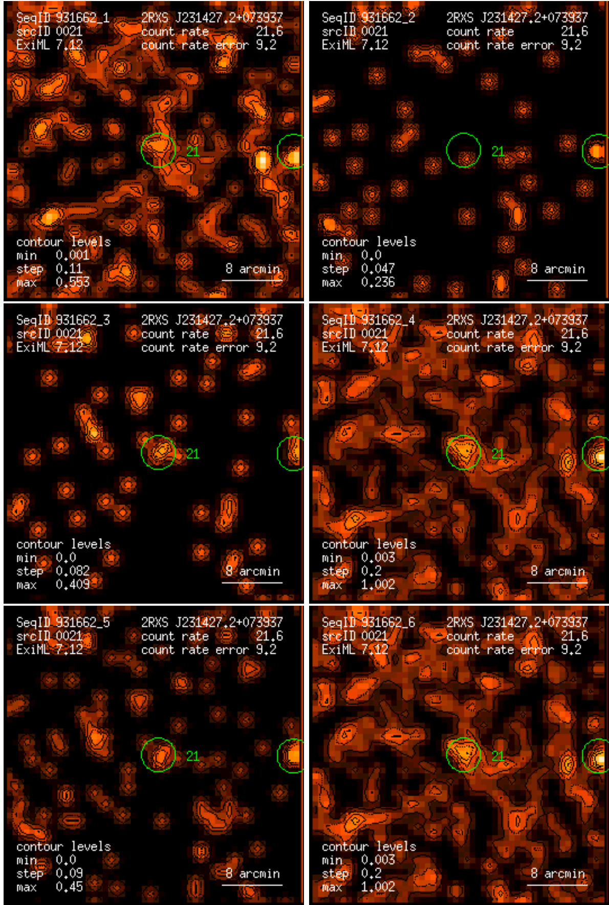
Figure 21: RASS 931662: detection 0021: band rate images, Gaussian filter: (1) PSPC channels 11 – 41, (2) 52 – 90, (3) 91 – 201, (4) 11 – 235, (5) 52 – 201, (6) 11 – 201. Broad band rates in counts/ks. Band rate contour levels in counts/ks/arcmin 2 .
