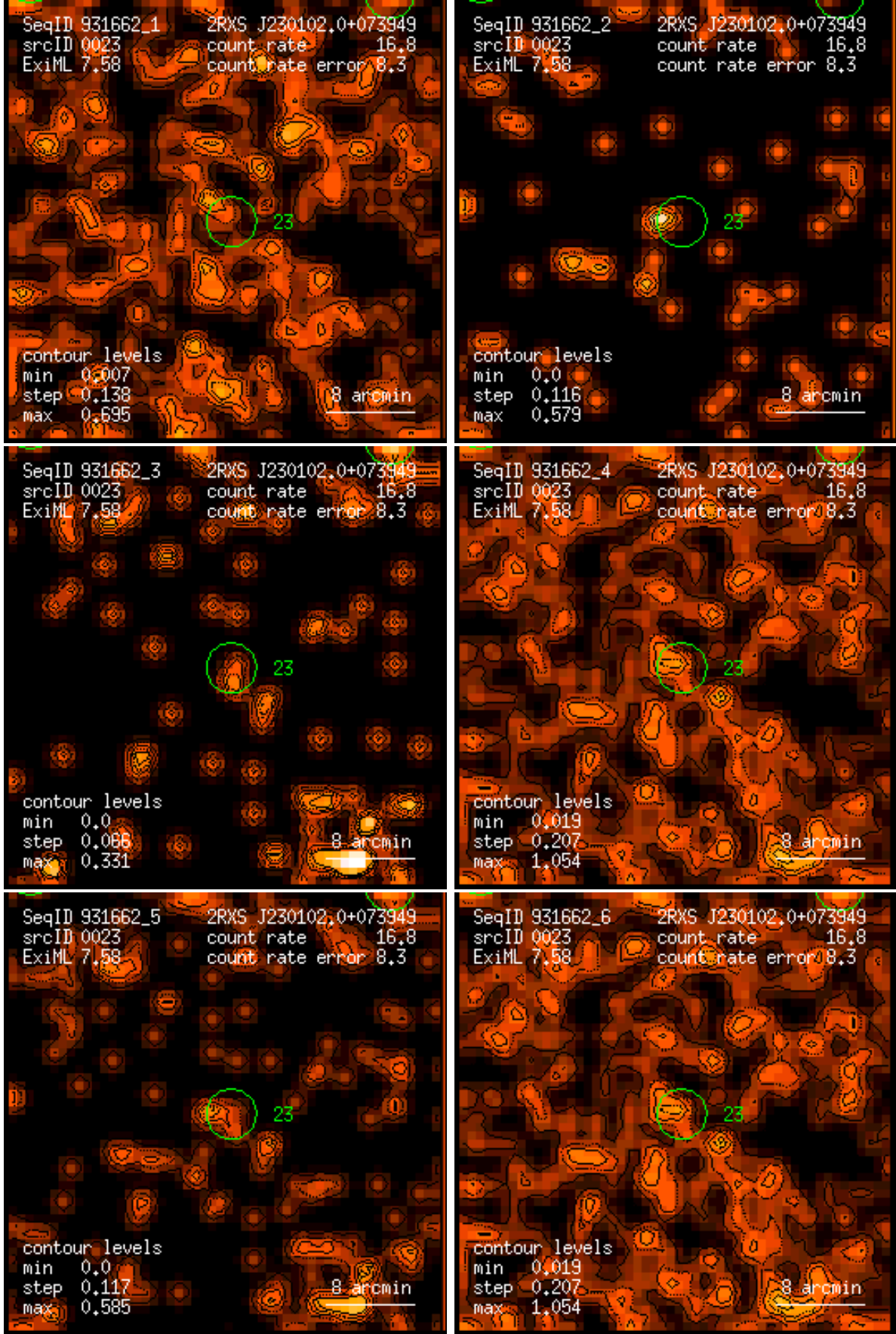
Figure 23: RASS 931662: detection 0023: band rate images, Gaussian filter: (1) PSPC channels 11 – 41, (2) 52 – 90, (3) 91 – 201, (4) 11 – 235, (5) 52 – 201, (6) 11 – 201. Broad band rates in counts/ks. Band rate contour levels in counts/ks/arcmin 2 .
