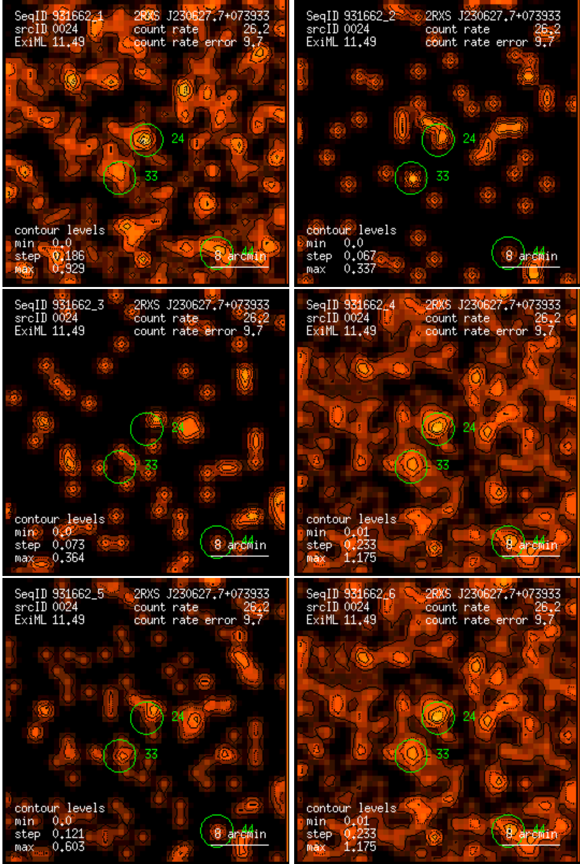
Figure 24: RASS 931662: detection 0024: band rate images, Gaussian filter: (1) PSPC channels 11 – 41, (2) 52 – 90, (3) 91 – 201, (4) 11 – 235, (5) 52 – 201, (6) 11 – 201. Broad band rates in counts/ks. Band rate contour levels in counts/ks/arcmin 2 .
