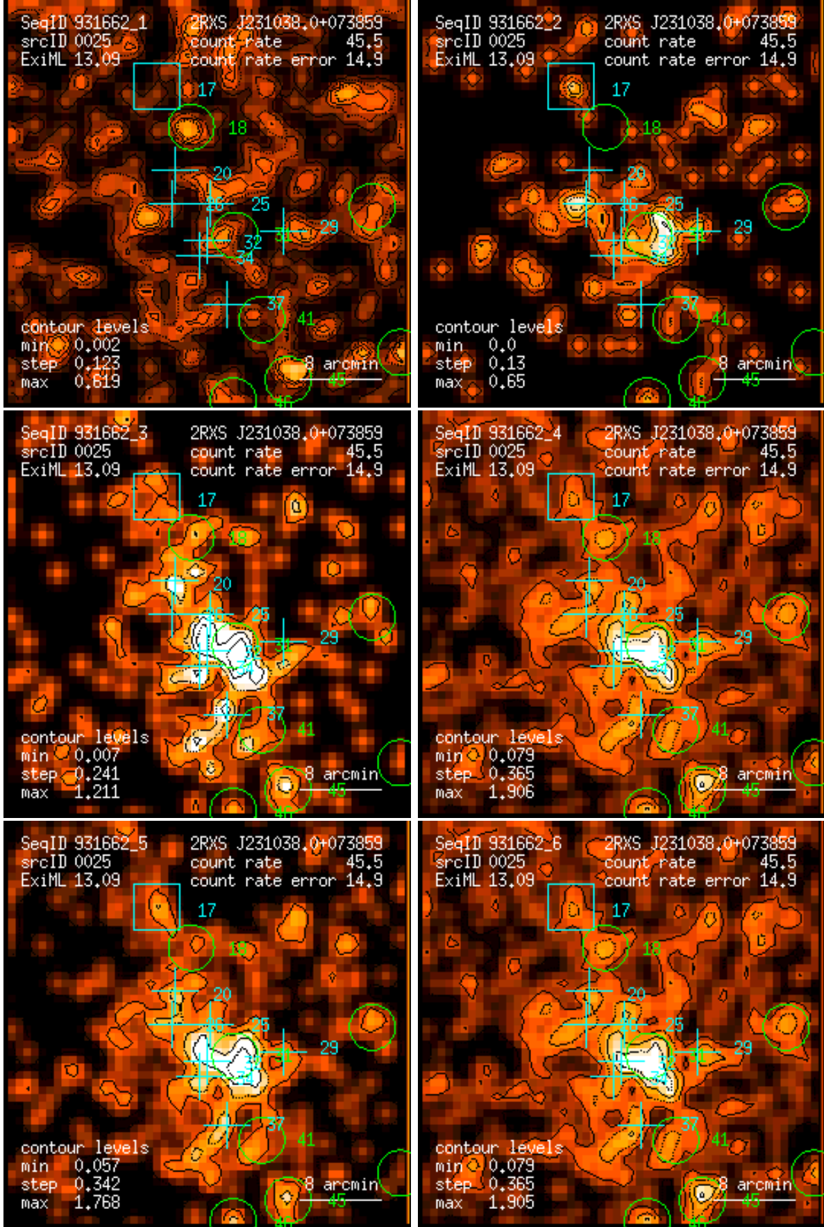
Figure 25: RASS 931662: detection 0025: band rate images, Gaussian filter: (1) PSPC channels 11 – 41, (2) 52 – 90, (3) 91 – 201, (4) 11 – 235, (5) 52 – 201, (6) 11 – 201. Broad band rates in counts/ks. Band rate contour levels in counts/ks/arcmin 2 .
