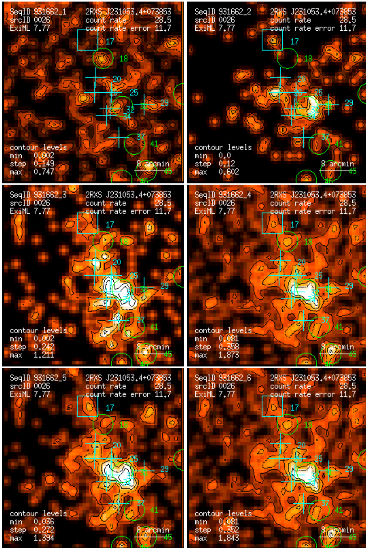
Figure 26: RASS 931662: detection 0026: band rate images, Gaussian filter: (1) PSPC channels 11 – 41, (2) 52 – 90, (3) 91 – 201, (4) 11 – 235, (5) 52 – 201, (6) 11 – 201. Broad band rates in counts/ks. Band rate contour levels in counts/ks/arcmin 2 .
