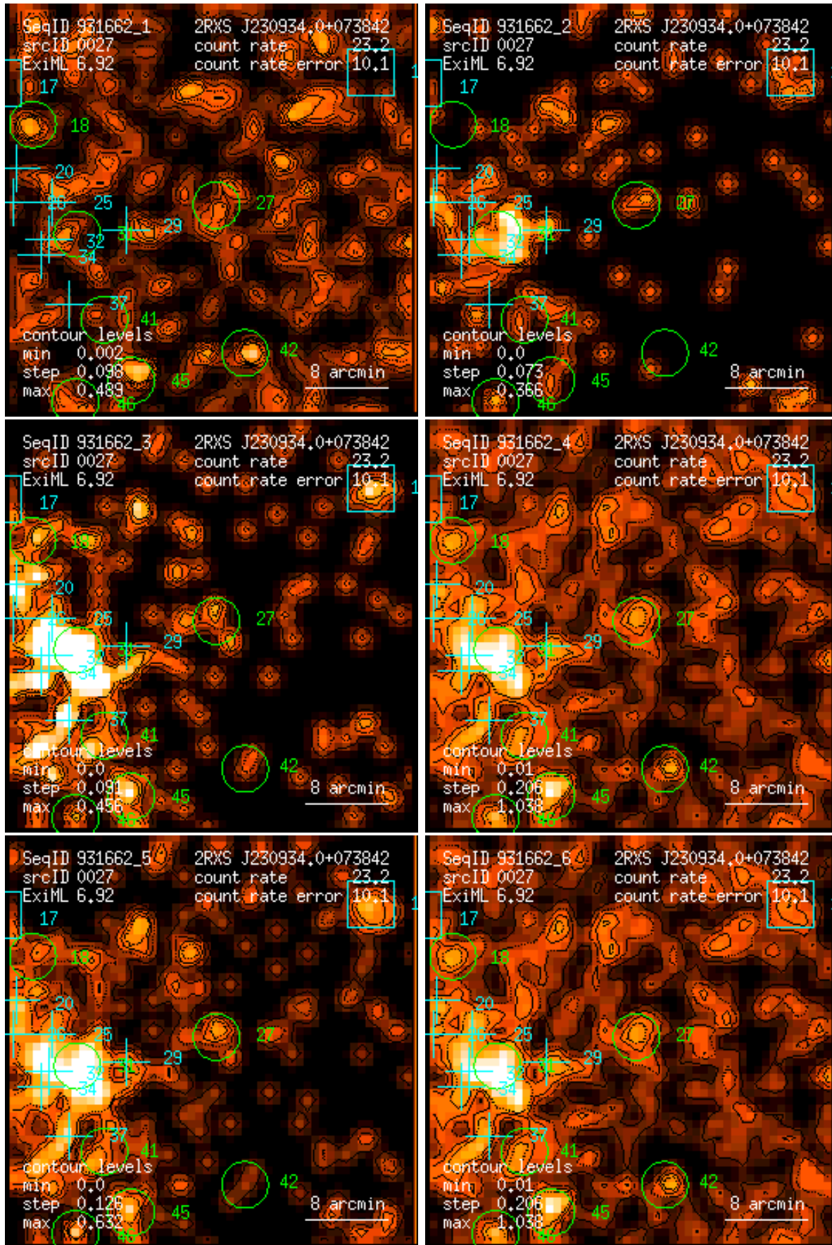
Figure 27: RASS 931662: detection 0027: band rate images, Gaussian filter: (1) PSPC channels 11 – 41, (2) 52 – 90, (3) 91 – 201, (4) 11 – 235, (5) 52 – 201, (6) 11 – 201. Broad band rates in counts/ks. Band rate contour levels in counts/ks/arcmin 2 .
