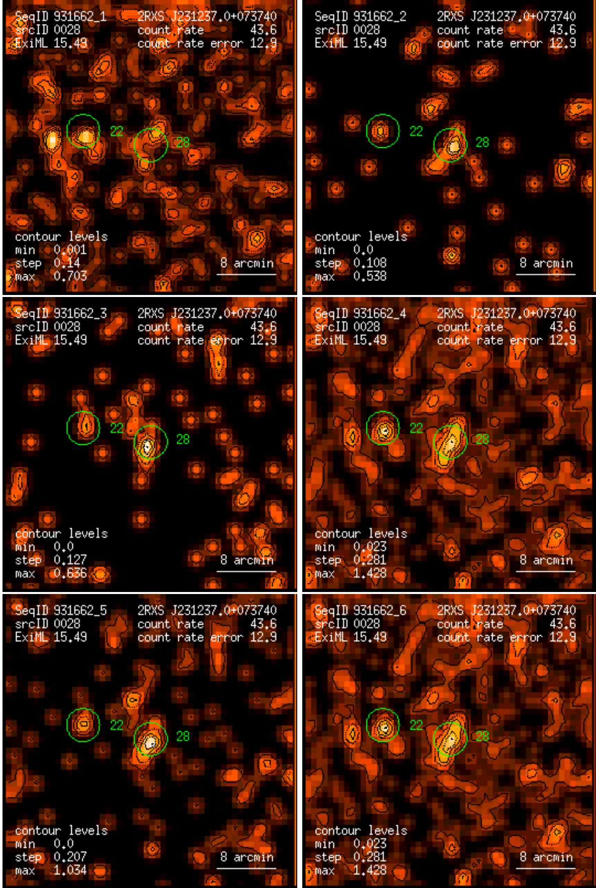
Figure 28: RASS 931662: detection 0028: band rate images, Gaussian filter: (1) PSPC channels 11 – 41, (2) 52 – 90, (3) 91 – 201, (4) 11 – 235, (5) 52 – 201, (6) 11 – 201. Broad band rates in counts/ks. Band rate contour levels in counts/ks/arcmin 2 .
