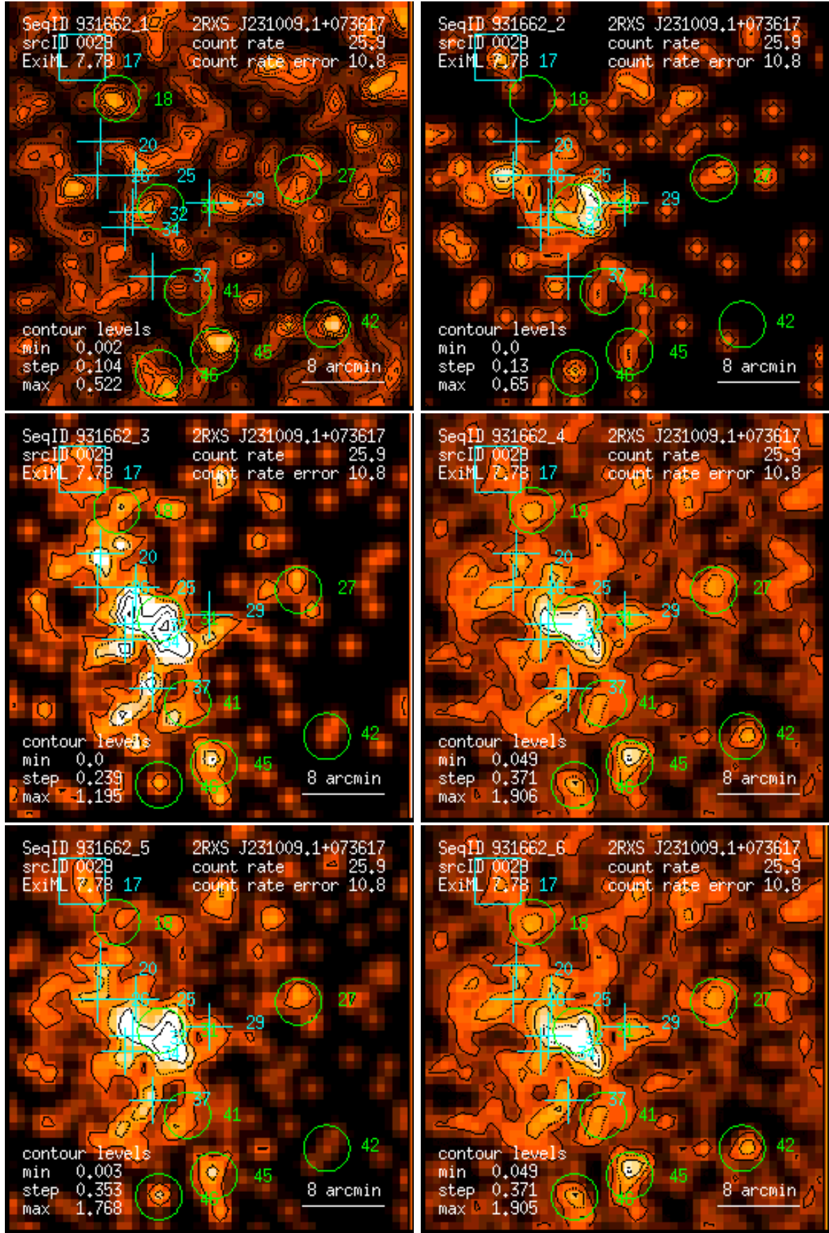
Figure 29: RASS 931662: detection 0029: band rate images, Gaussian filter: (1) PSPC channels 11 – 41, (2) 52 – 90, (3) 91 – 201, (4) 11 – 235, (5) 52 – 201, (6) 11 – 201. Broad band rates in counts/ks. Band rate contour levels in counts/ks/arcmin 2 .
