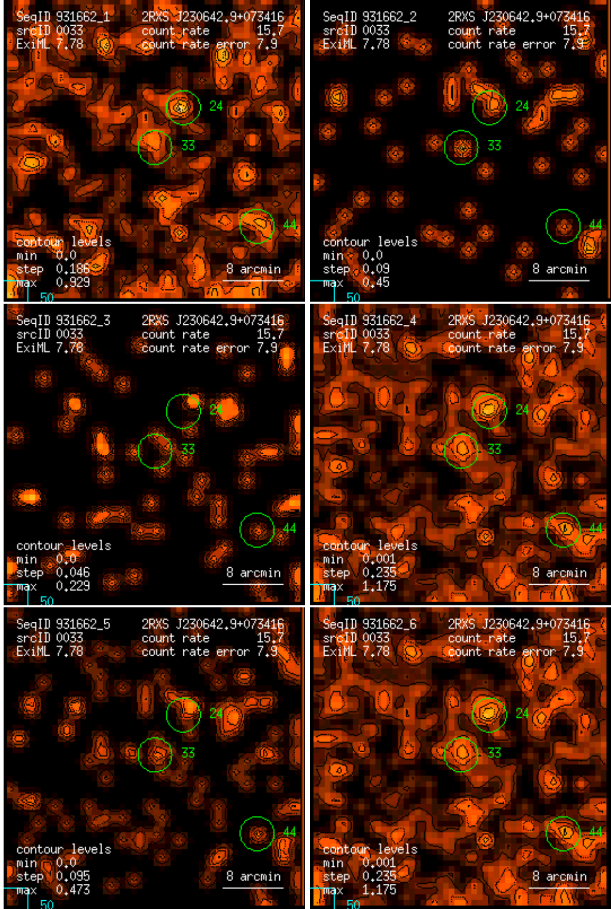
Figure 33: RASS 931662: detection 0033: band rate images, Gaussian filter: (1) PSPC channels 11 – 41, (2) 52 – 90, (3) 91 – 201, (4) 11 – 235, (5) 52 – 201, (6) 11 – 201. Broad band rates in counts/ks. Band rate contour levels in counts/ks/arcmin 2 .
