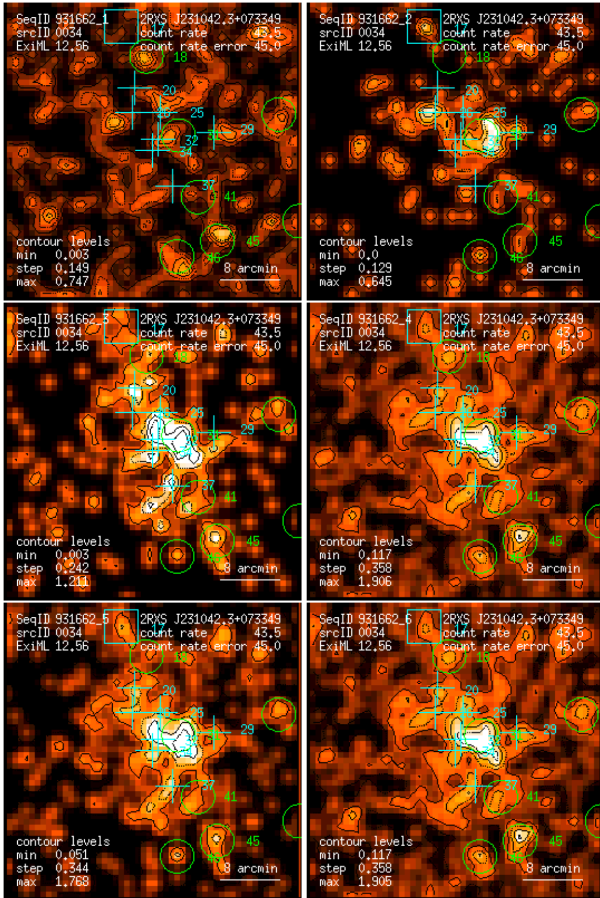
Figure 34: RASS 931662: detection 0034: band rate images, Gaussian filter: (1) PSPC channels 11 – 41, (2) 52 – 90, (3) 91 – 201, (4) 11 – 235, (5) 52 – 201, (6) 11 – 201. Broad band rates in counts/ks. Band rate contour levels in counts/ks/arcmin 2 .
