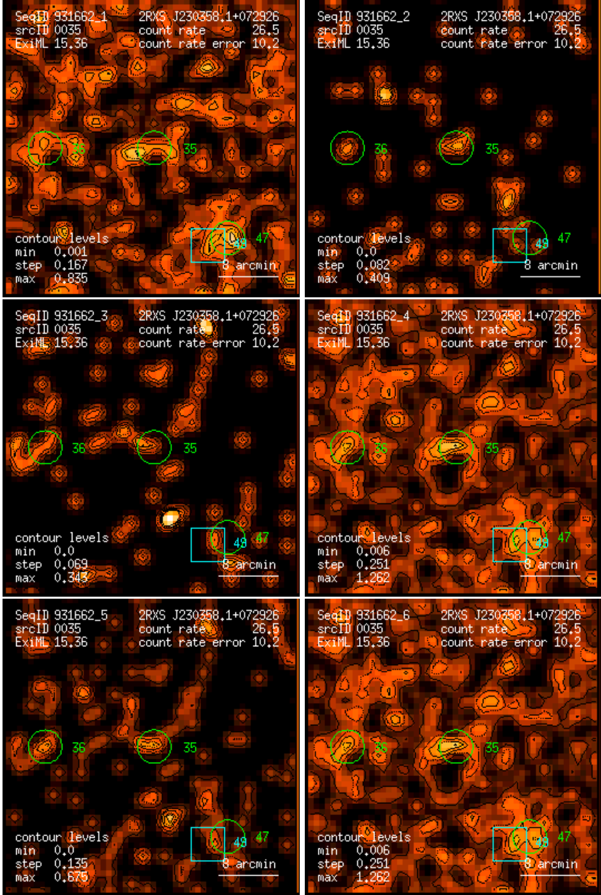
Figure 35: RASS 931662: detection 0035: band rate images, Gaussian filter: (1) PSPC channels 11 – 41, (2) 52 – 90, (3) 91 – 201, (4) 11 – 235, (5) 52 – 201, (6) 11 – 201. Broad band rates in counts/ks. Band rate contour levels in counts/ks/arcmin 2 .
