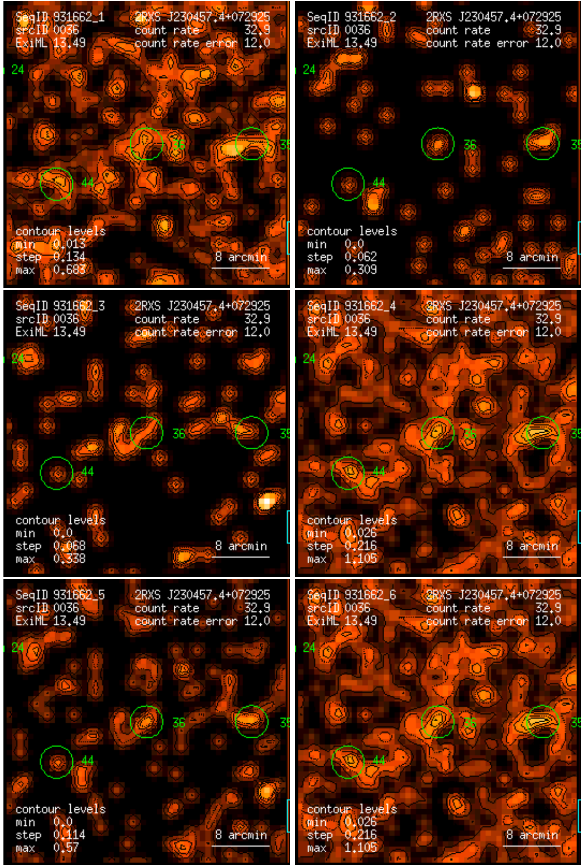
Figure 36: RASS 931662: detection 0036: band rate images, Gaussian filter: (1) PSPC channels 11 – 41, (2) 52 – 90, (3) 91 – 201, (4) 11 – 235, (5) 52 – 201, (6) 11 – 201. Broad band rates in counts/ks. Band rate contour levels in counts/ks/arcmin 2 .
