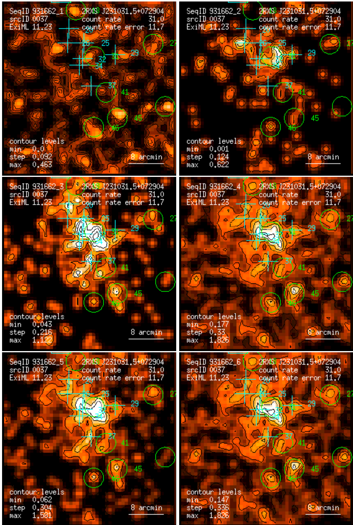
Figure 37: RASS 931662: detection 0037: band rate images, Gaussian filter: (1) PSPC channels 11 – 41, (2) 52 – 90, (3) 91 – 201, (4) 11 – 235, (5) 52 – 201, (6) 11 – 201. Broad band rates in counts/ks. Band rate contour levels in counts/ks/arcmin 2 .
