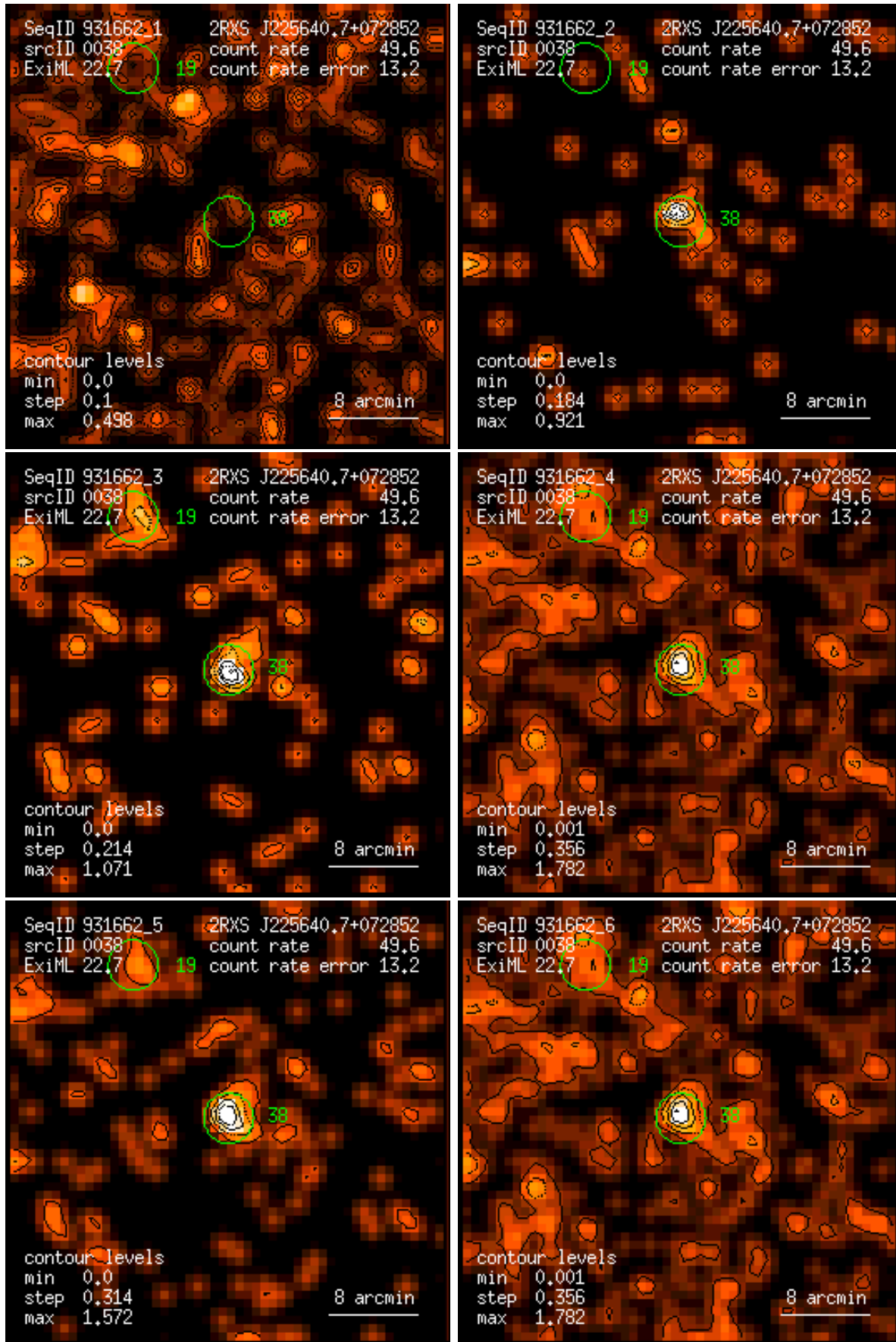
Figure 38: RASS 931662: detection 0038: band rate images, Gaussian filter: (1) PSPC channels 11 – 41, (2) 52 – 90, (3) 91 – 201, (4) 11 – 235, (5) 52 – 201, (6) 11 – 201. Broad band rates in counts/ks. Band rate contour levels in counts/ks/arcmin 2 .
