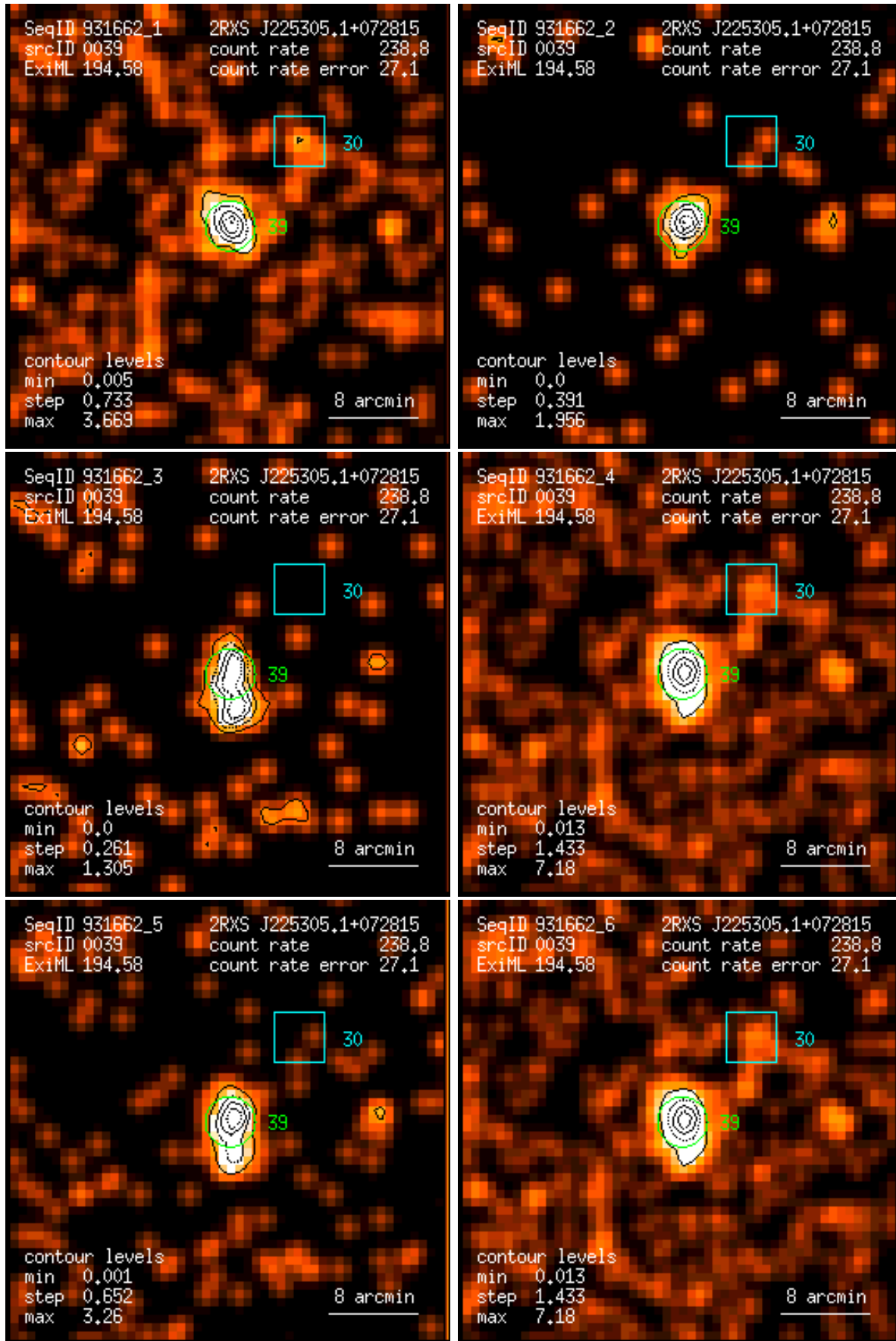
Figure 39: RASS 931662: detection 0039: band rate images, Gaussian filter: (1) PSPC channels 11 – 41, (2) 52 – 90, (3) 91 – 201, (4) 11 – 235, (5) 52 – 201, (6) 11 – 201. Broad band rates in counts/ks. Band rate contour levels in counts/ks/arcmin 2 .
