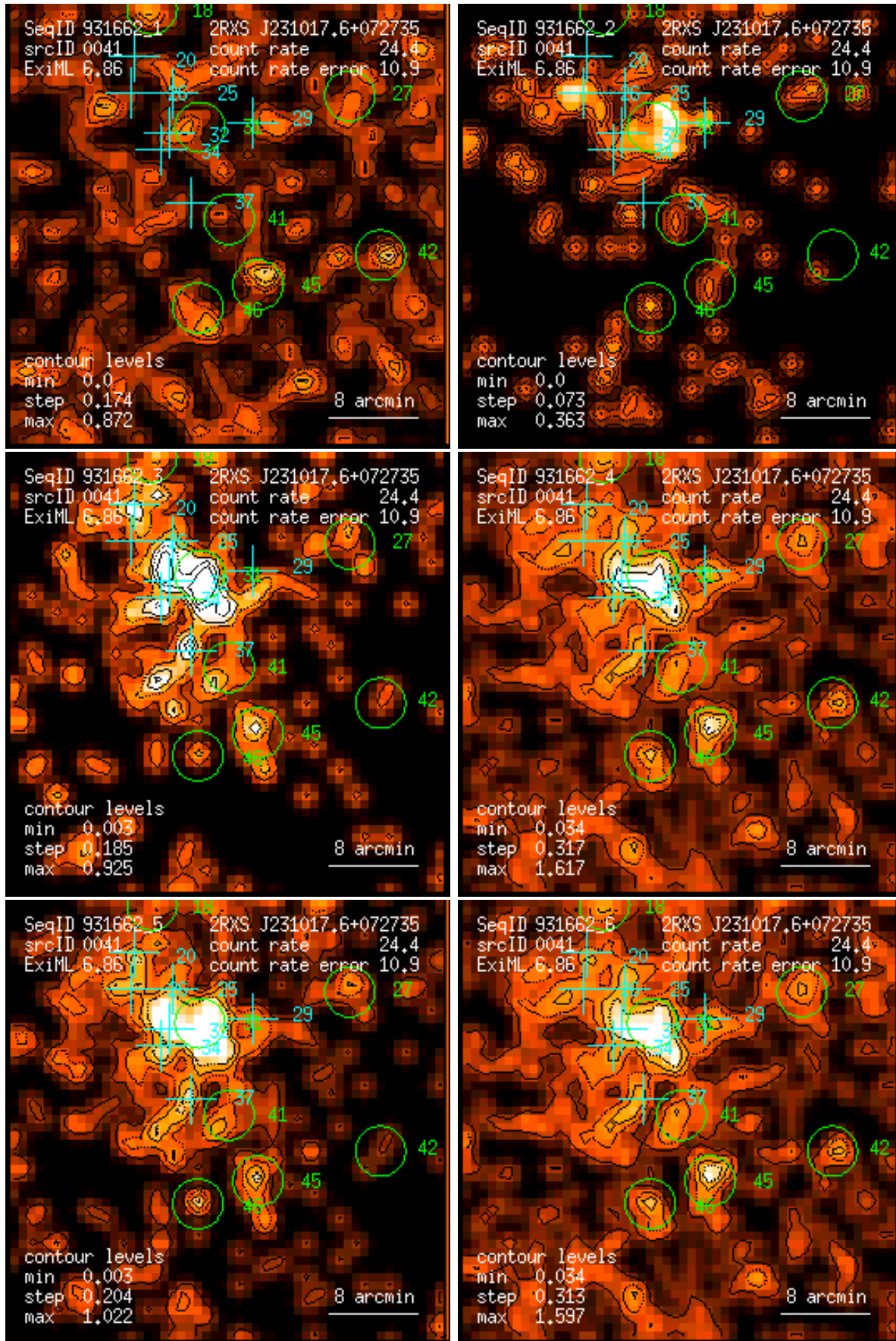
Figure 41: RASS 931662: detection 0041: band rate images, Gaussian filter: (1) PSPC channels 11 – 41, (2) 52 – 90, (3) 91 – 201, (4) 11 – 235, (5) 52 – 201, (6) 11 – 201. Broad band rates in counts/ks. Band rate contour levels in counts/ks/arcmin 2 .
