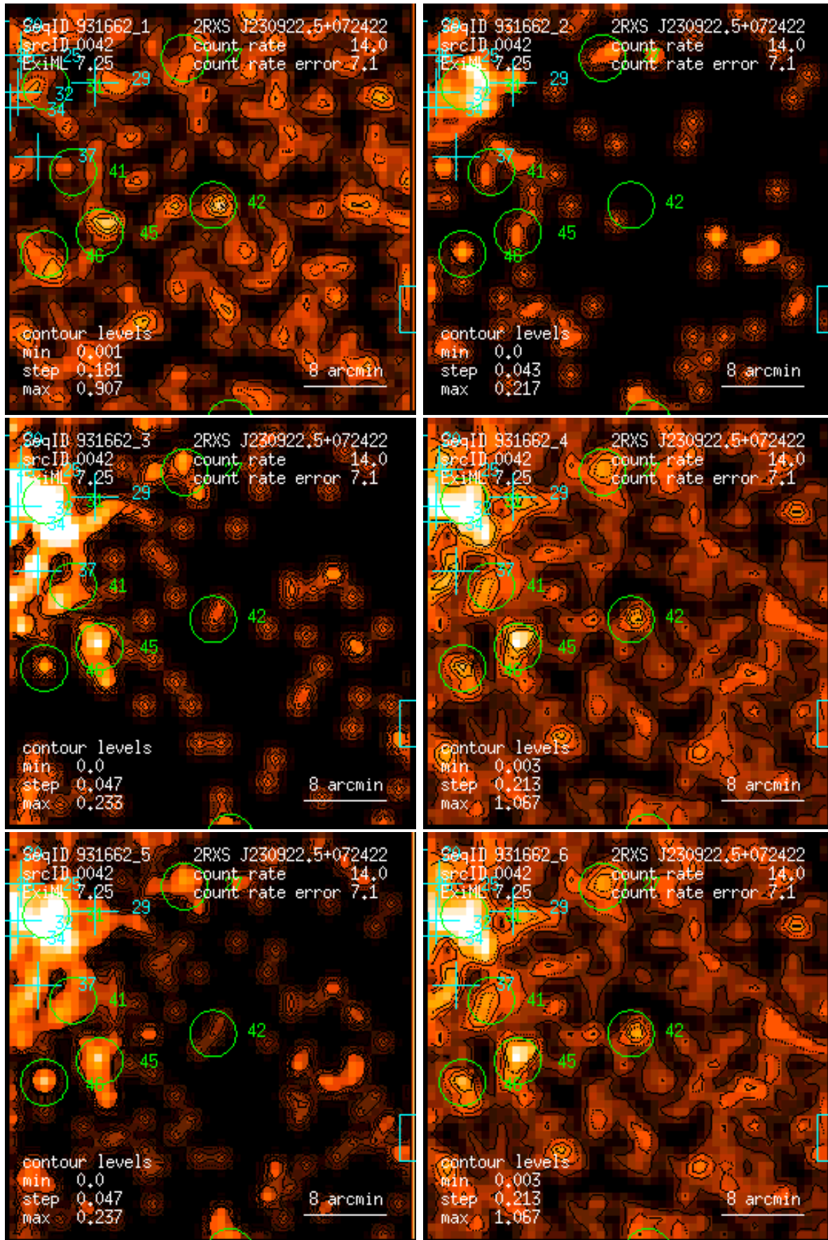
Figure 42: RASS 931662: detection 0042: band rate images, Gaussian filter: (1) PSPC channels 11 – 41, (2) 52 – 90, (3) 91 – 201, (4) 11 – 235, (5) 52 – 201, (6) 11 – 201. Broad band rates in counts/ks. Band rate contour levels in counts/ks/arcmin 2 .
