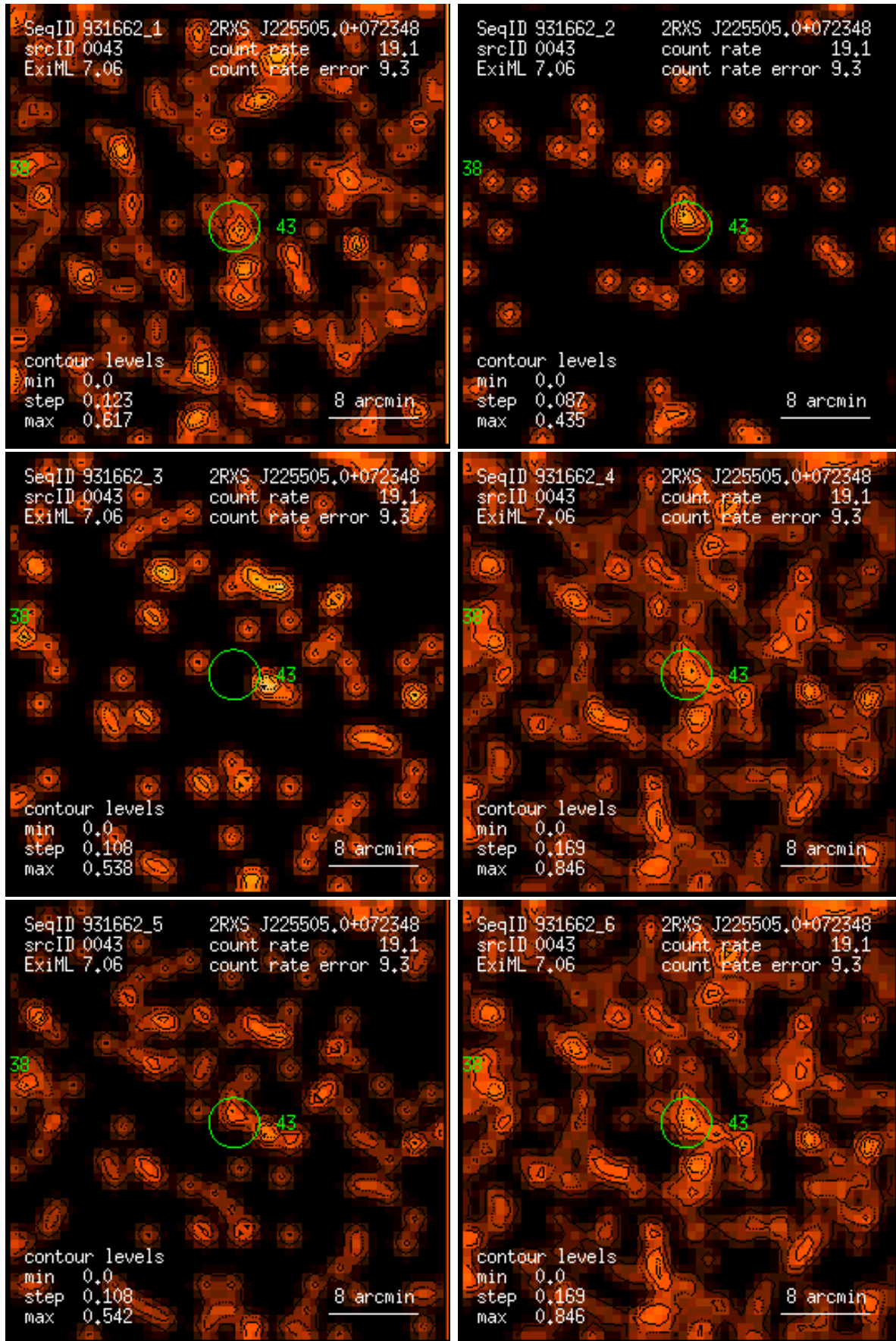
Figure 43: RASS 931662: detection 0043: band rate images, Gaussian filter: (1) PSPC channels 11 – 41, (2) 52 – 90, (3) 91 – 201, (4) 11 – 235, (5) 52 – 201, (6) 11 – 201. Broad band rates in counts/ks. Band rate contour levels in counts/ks/arcmin 2 .
