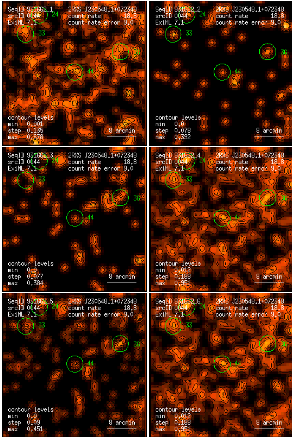
Figure 44: RASS 931662: detection 0044: band rate images, Gaussian filter: (1) PSPC channels 11 – 41, (2) 52 – 90, (3) 91 – 201, (4) 11 – 235, (5) 52 – 201, (6) 11 – 201. Broad band rates in counts/ks. Band rate contour levels in counts/ks/arcmin 2 .
